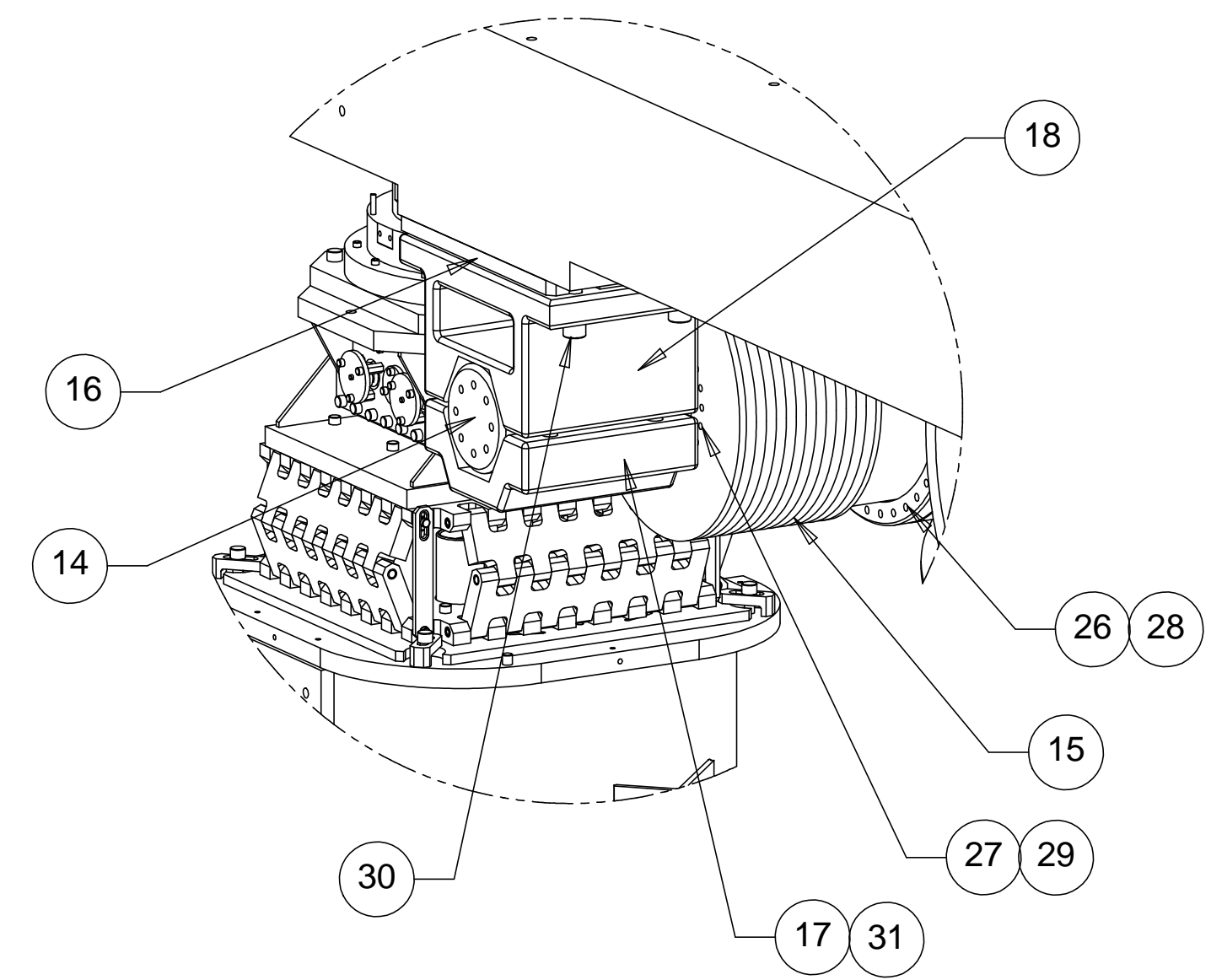
DETAIL B
