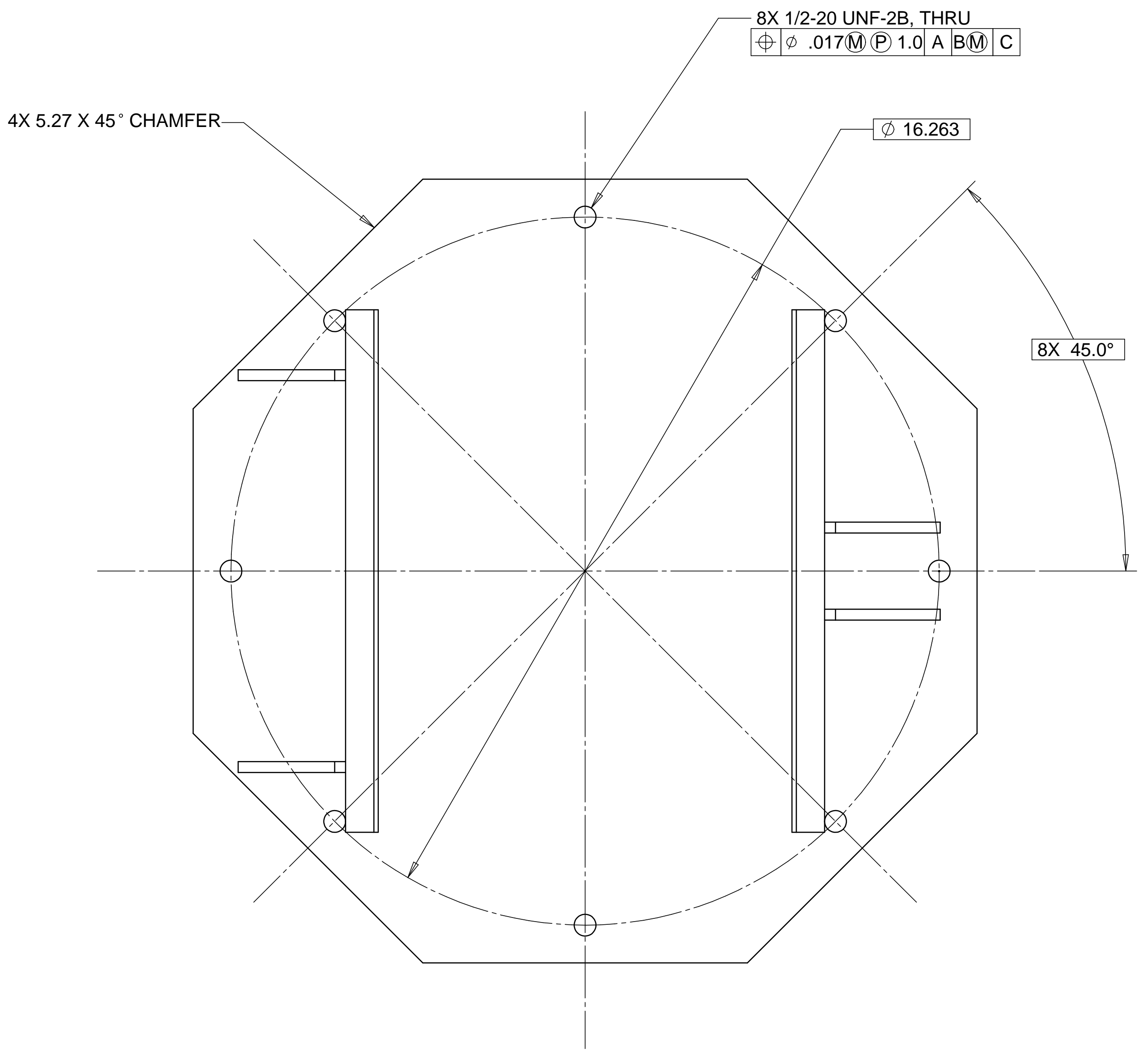
VIEW A - A FROM SHEET 1
