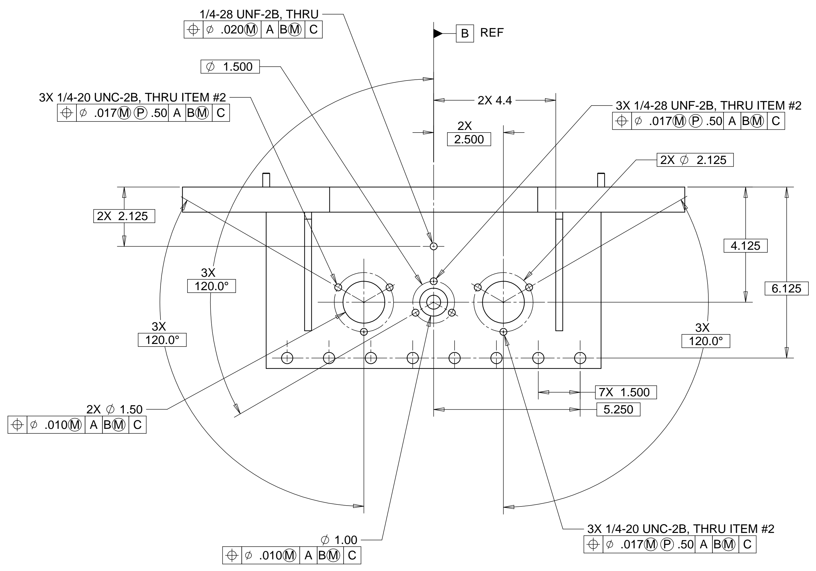
VIEW B - B FROM SHEET 1
