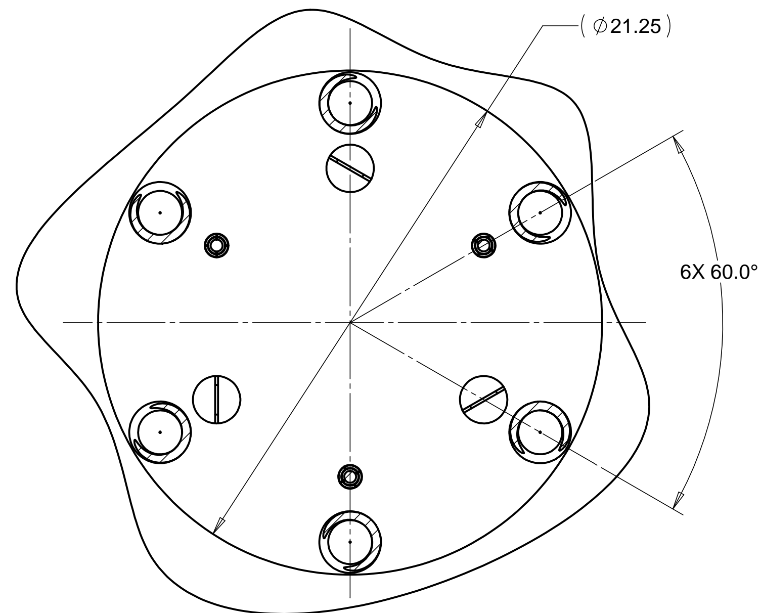
VIEW C-C
