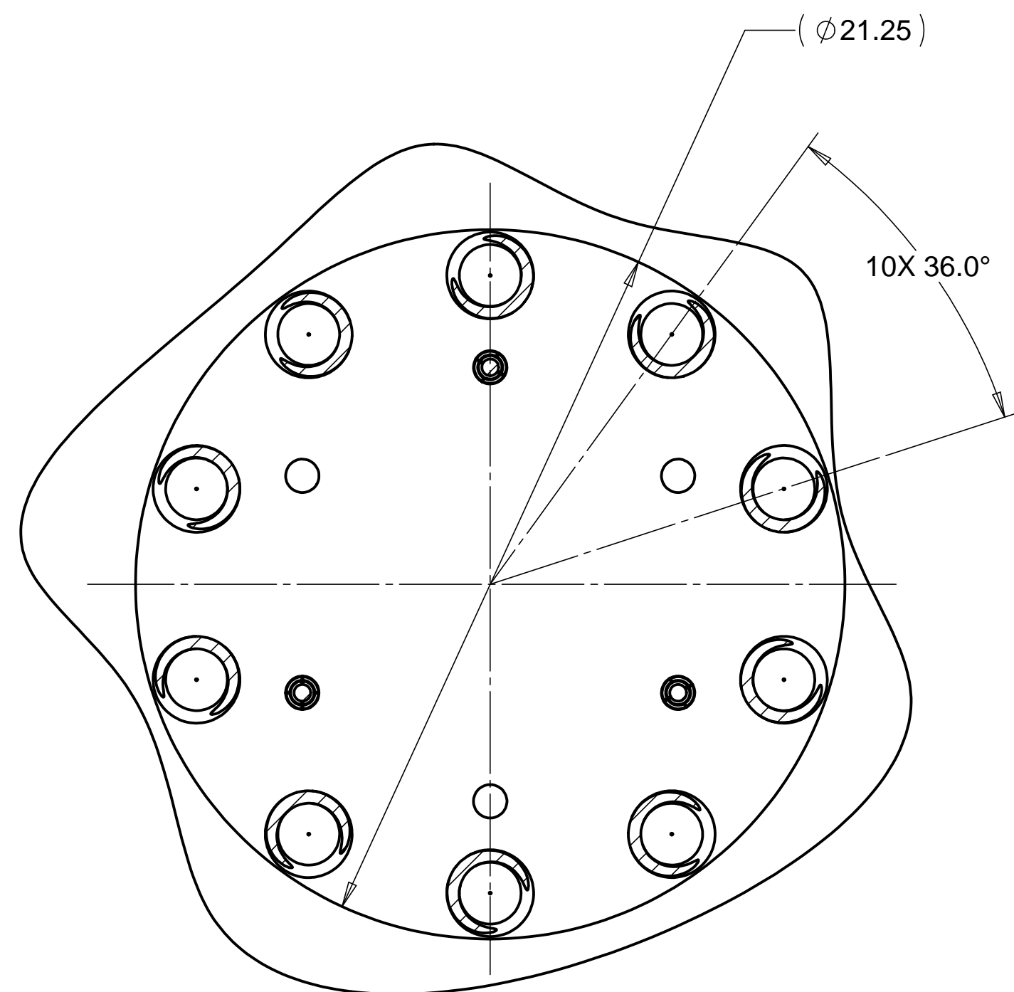
VIEW B-B
