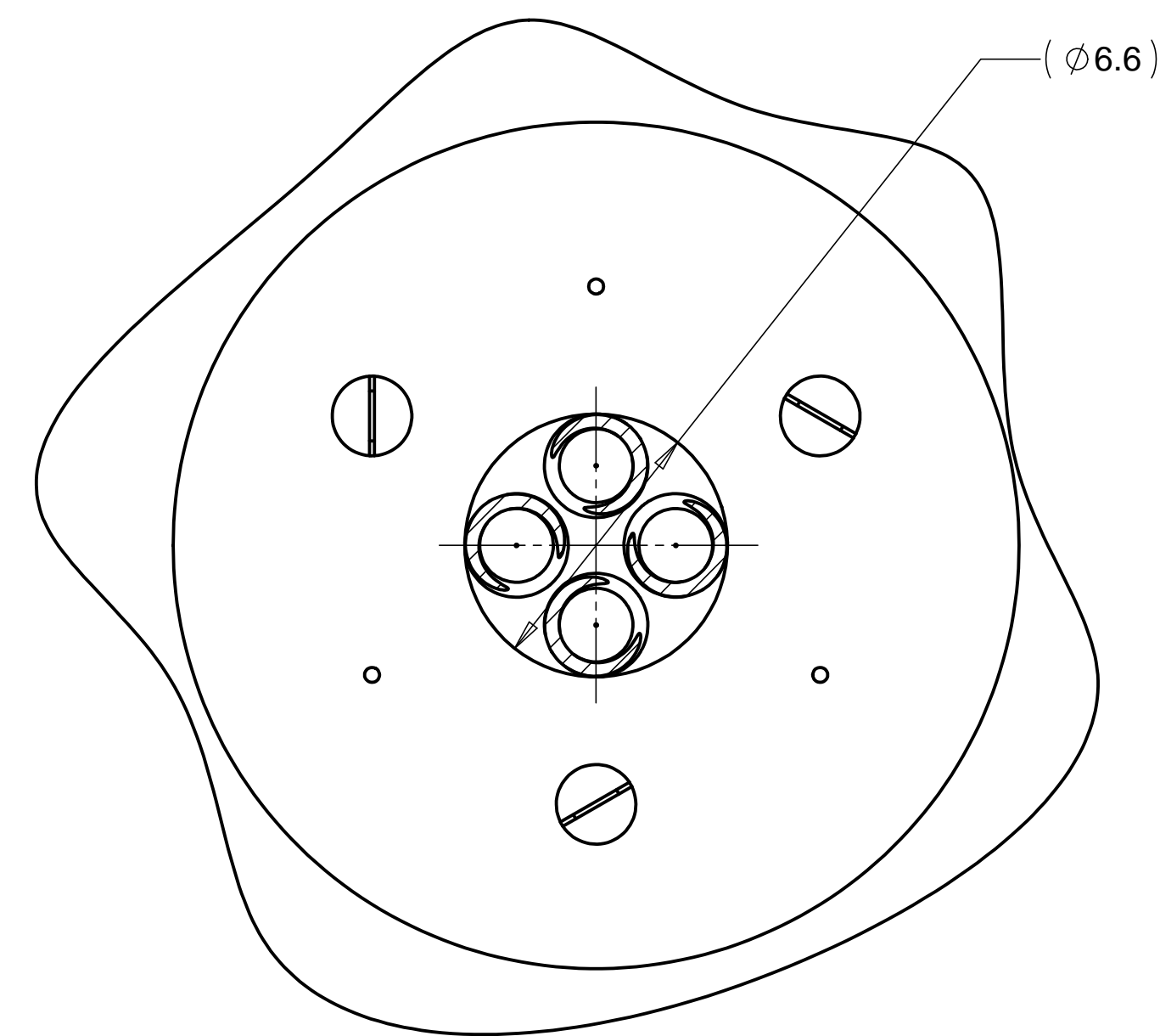
VIEW D-D
