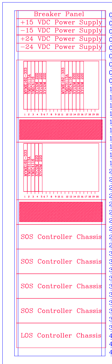
RACK 2X4
