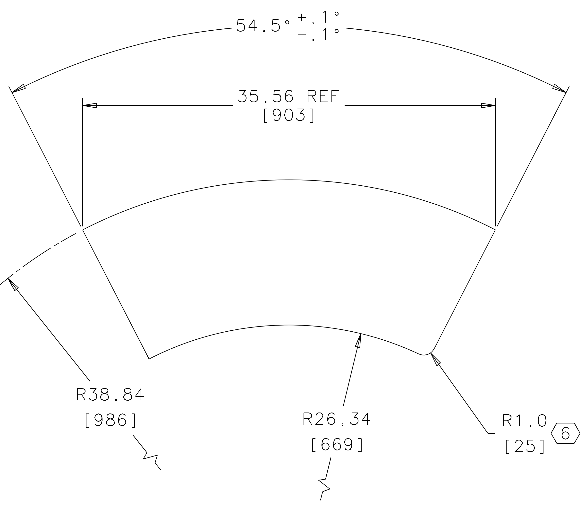
① & ② CONE SECTIONS ⑭
