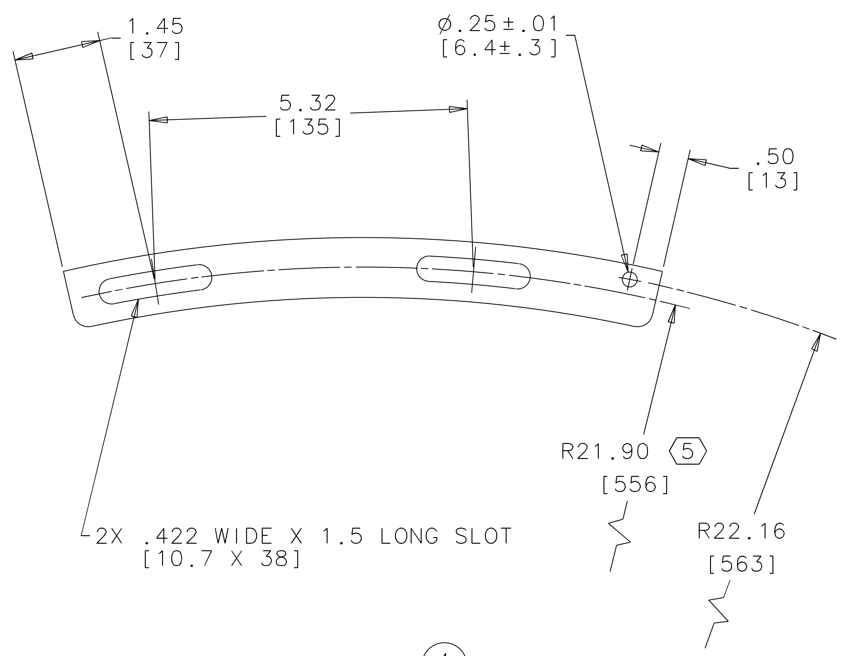
④ SLOTTED TAB (SAME AS ③ EXCEPT AS NOTED)
