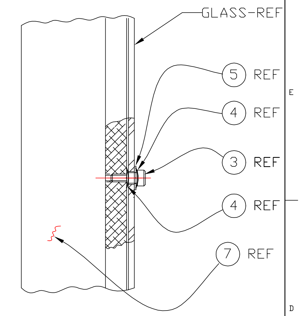
TYPICAL ASSEMBLY AT POINT OF GLASS SUPPORT ASSEMBLY AND GLASS PLATES
