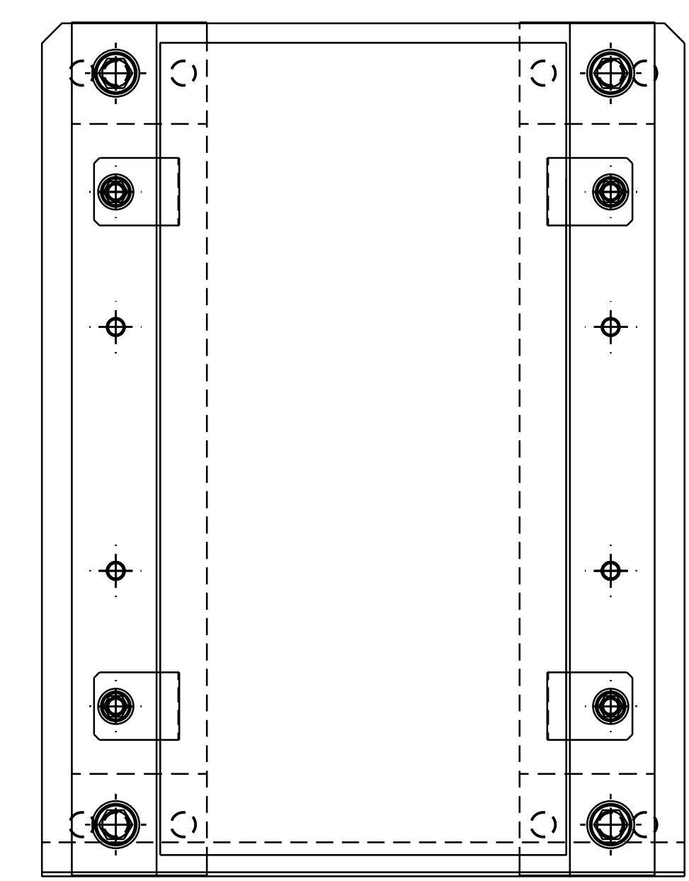
BEAM DUMP ASSEMBLY WITH 3" X 6" GLASS
