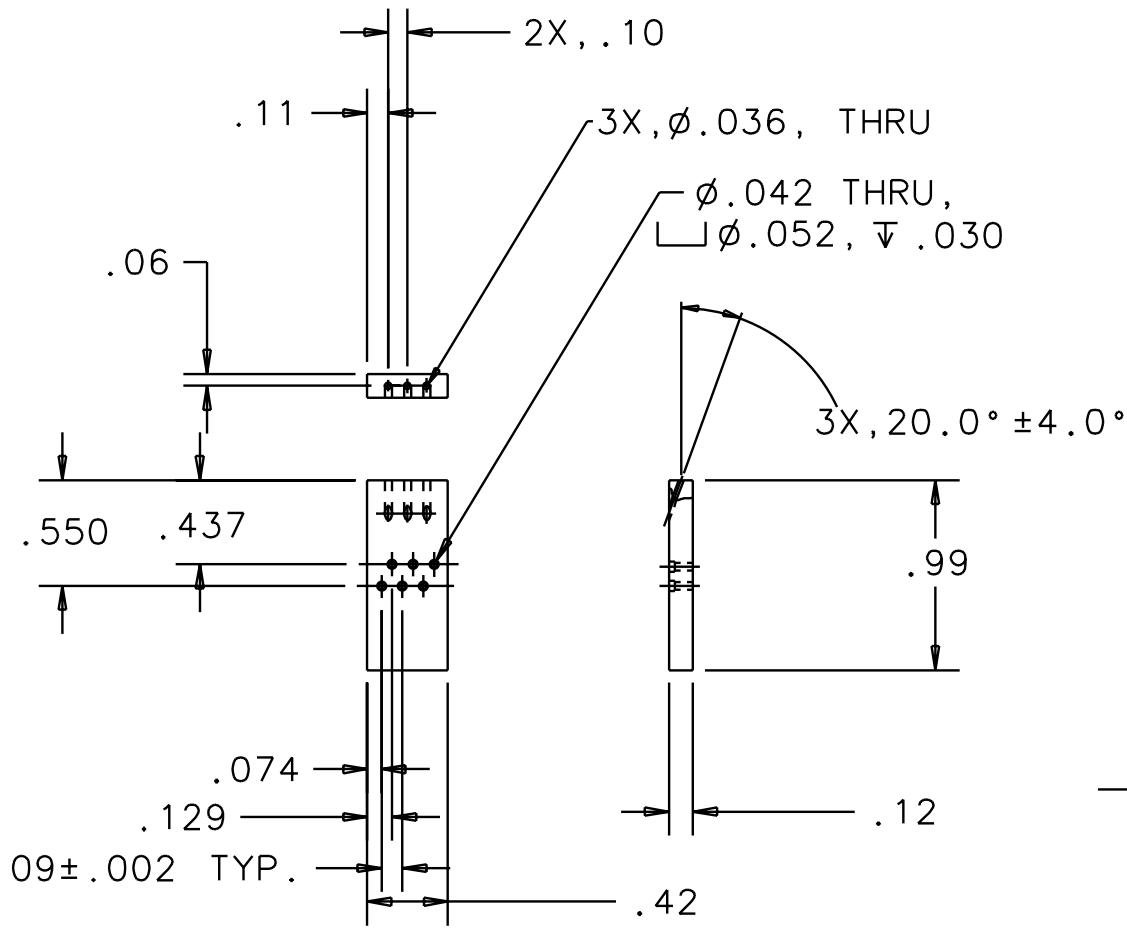
PIGTAIL RECTANGULAR PLATE DETAIL, ITEM 2 SCALE: 1/1
