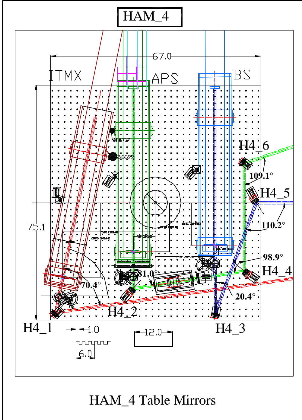
Figure 5: PO Telescopes 4K ITMx, 4K BS, 4K APS orientation
