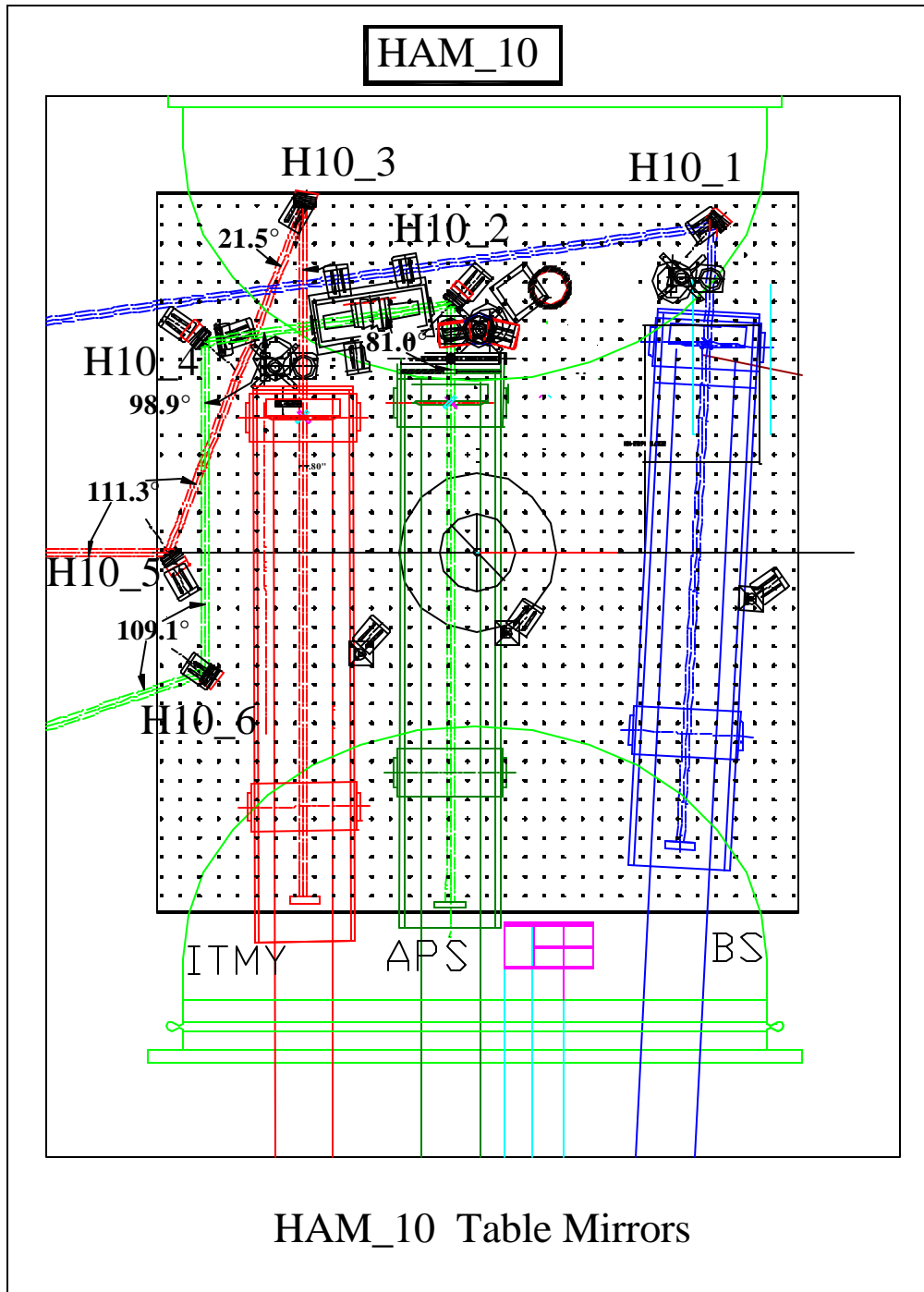
Figure 7: PO Telescopes 2K ITMy, 2K BS, 2K APS orientation
