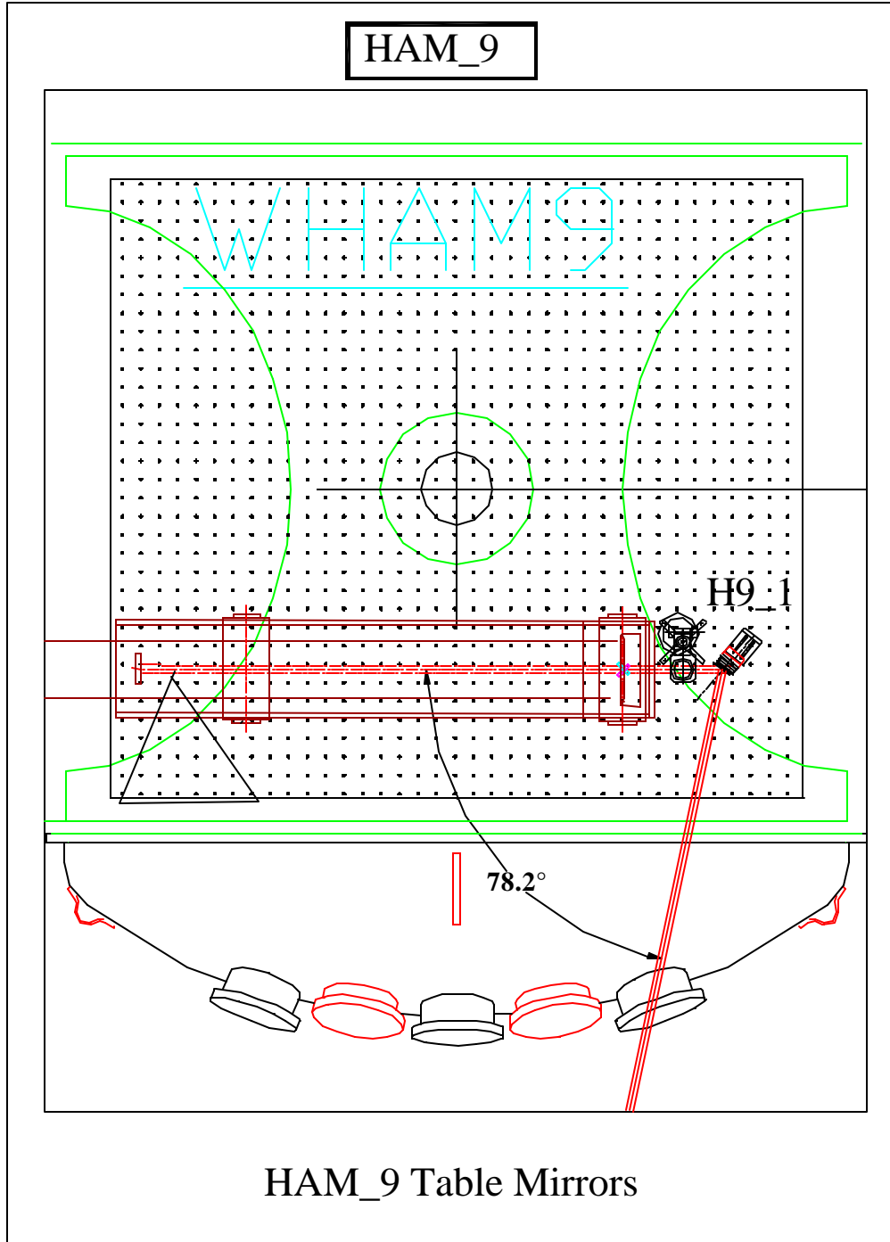
Figure 6: PO Telescope 2K ITMx, orientation
