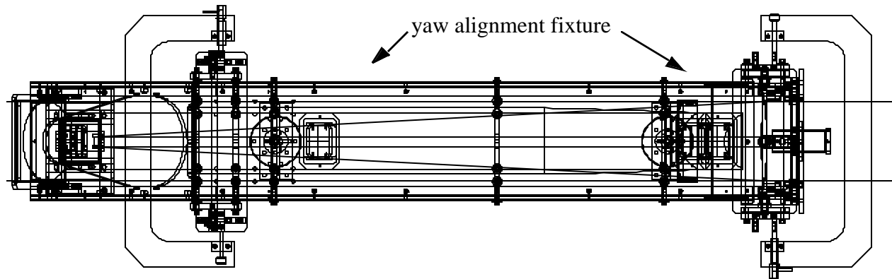
Figure 3: PO Telescope, top view
