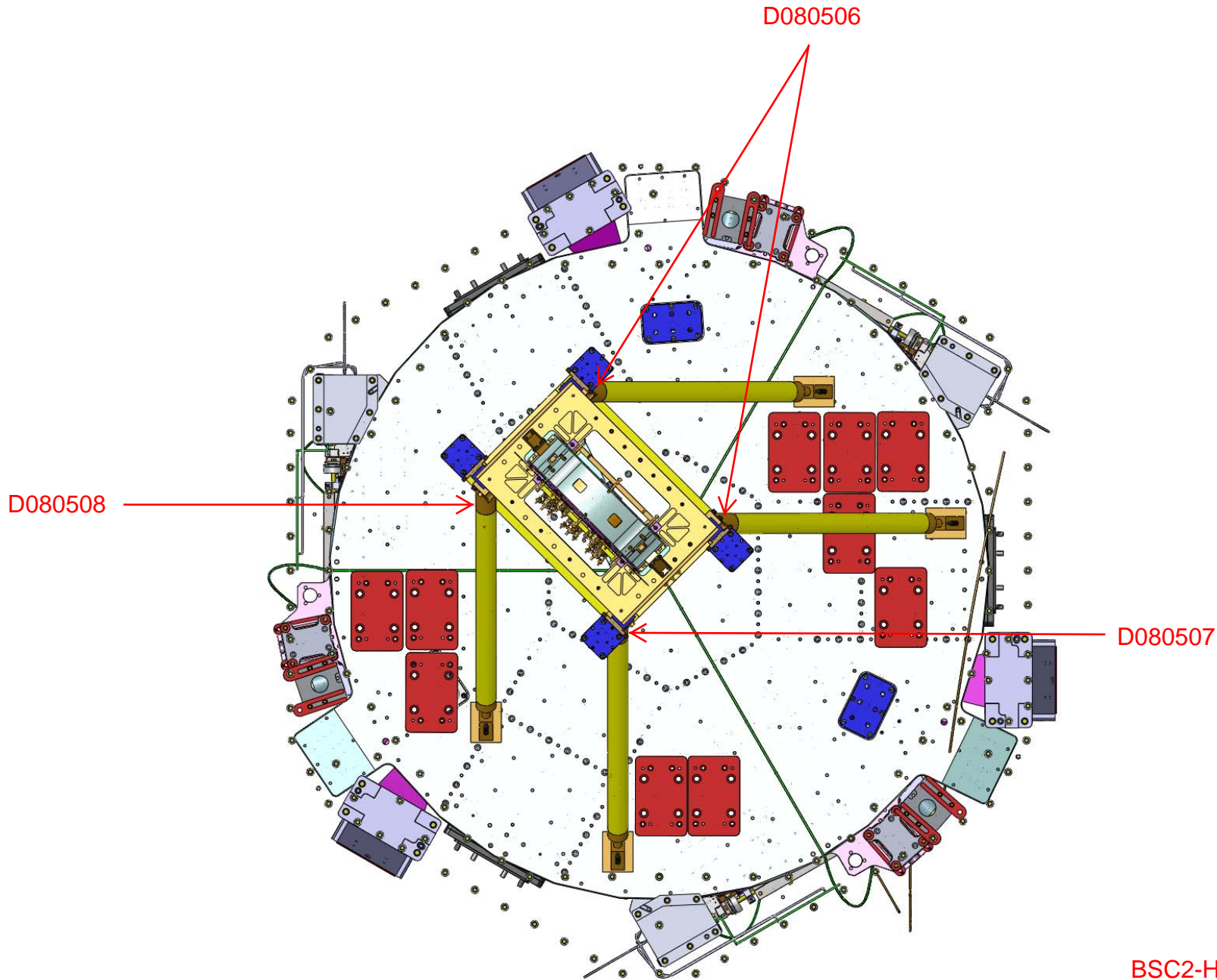
(D1000392 CONFIGURATION "BS FULL STAY POSITIONS BSC2-H1, L1") (D080501 CONFIGURATION "STAY POSITIONS H1, L1")
