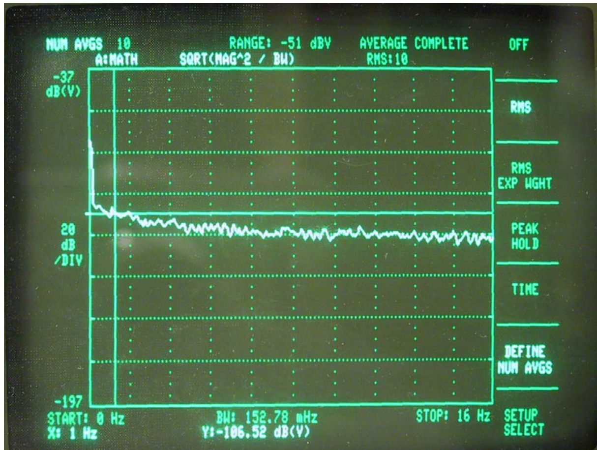
Figure 6. Noise spectrum for the OSEM under test, when connected to the Interface electronics.
