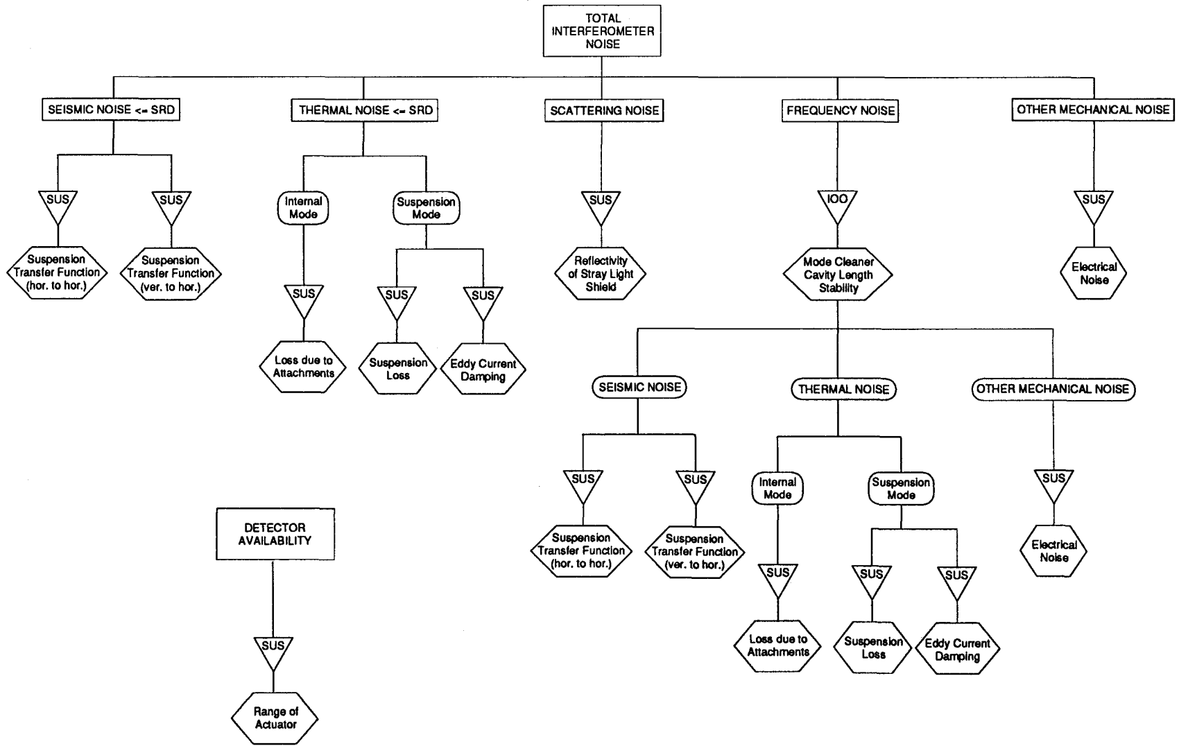
Figure 1: Interferometer Requirements Flowdown to SUS
