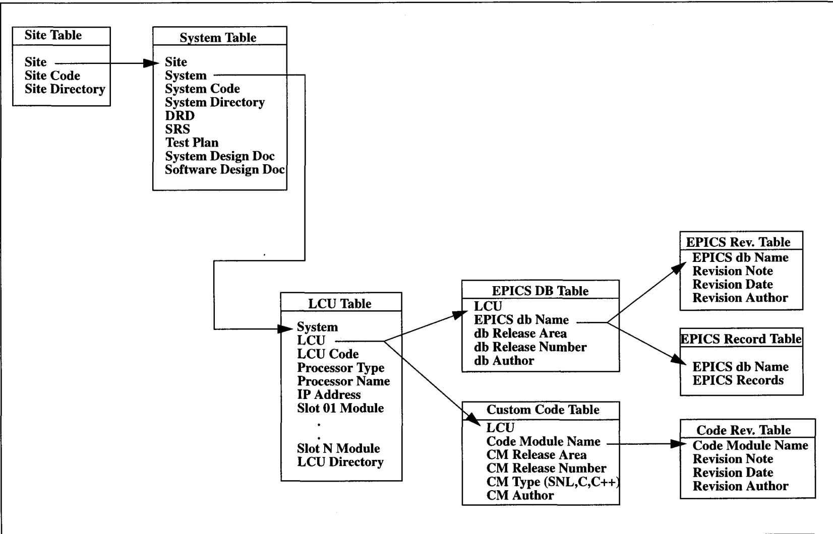
Figure 4: CDS EPICS Database Tables
