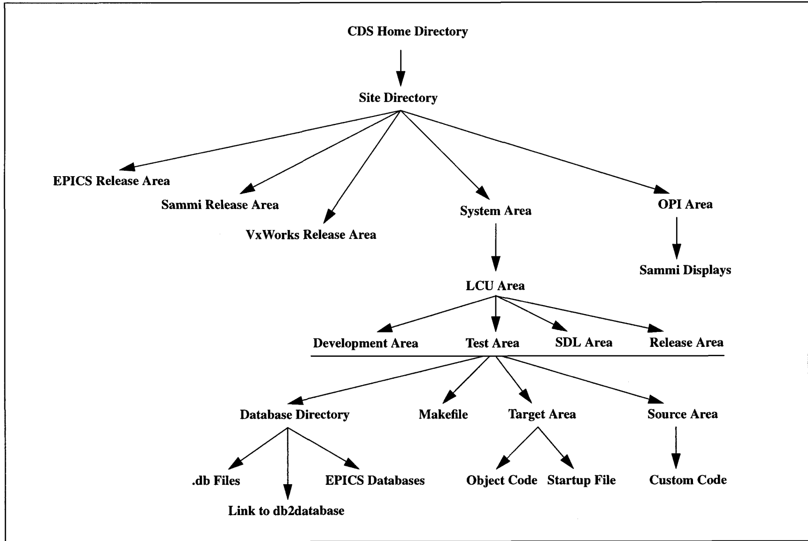
Figure 5: CDS Software Directory Structure
