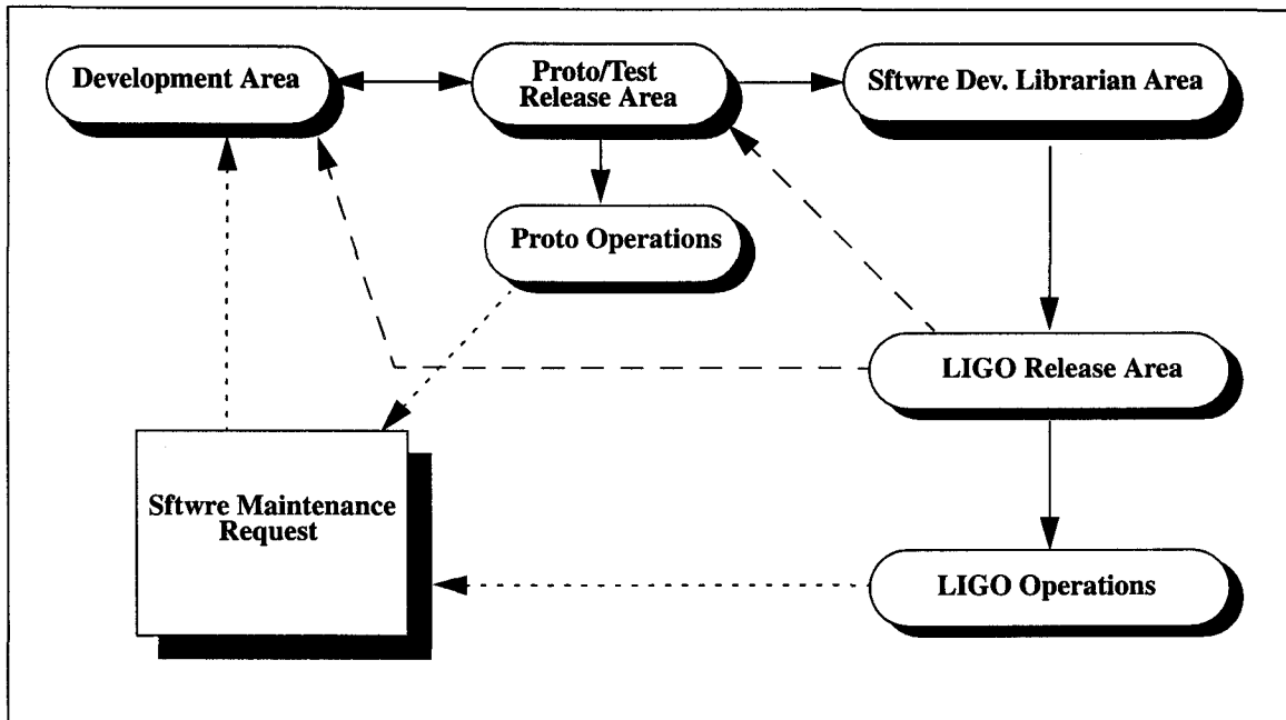
Figure 1: Software Configuration Control Flow
