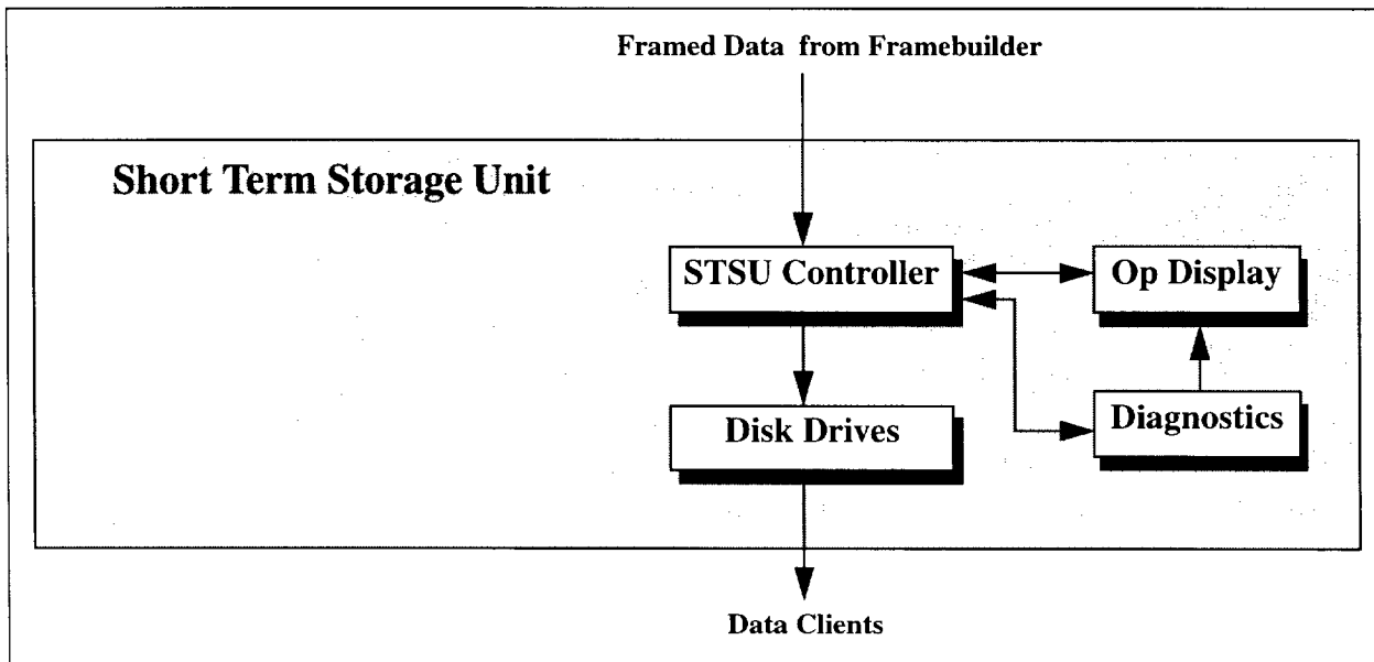
Figure 8: STSU Block Diagram
