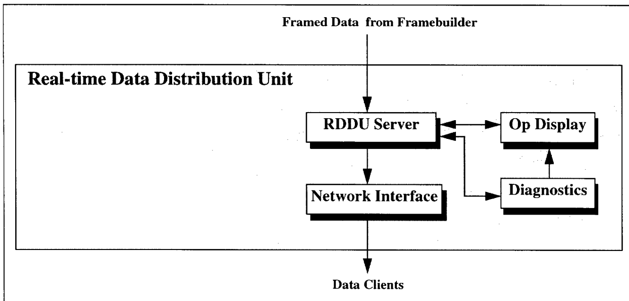
Figure 9: RDDU Block Diagram
