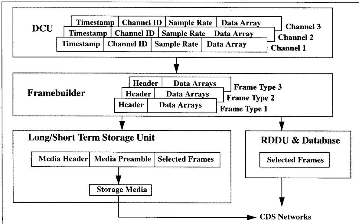
Figure 4: Data Flow Concept
