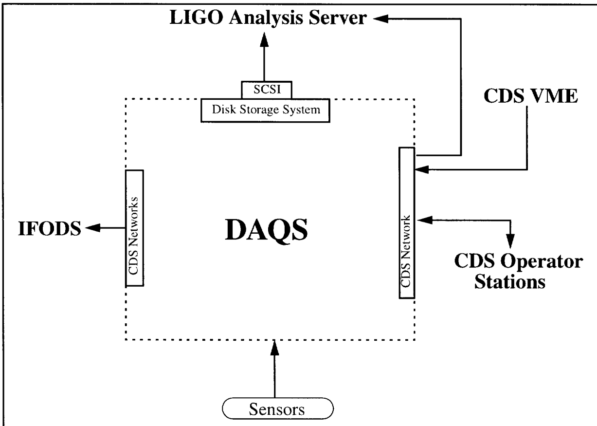
Figure 2: DAQS Interfaces
