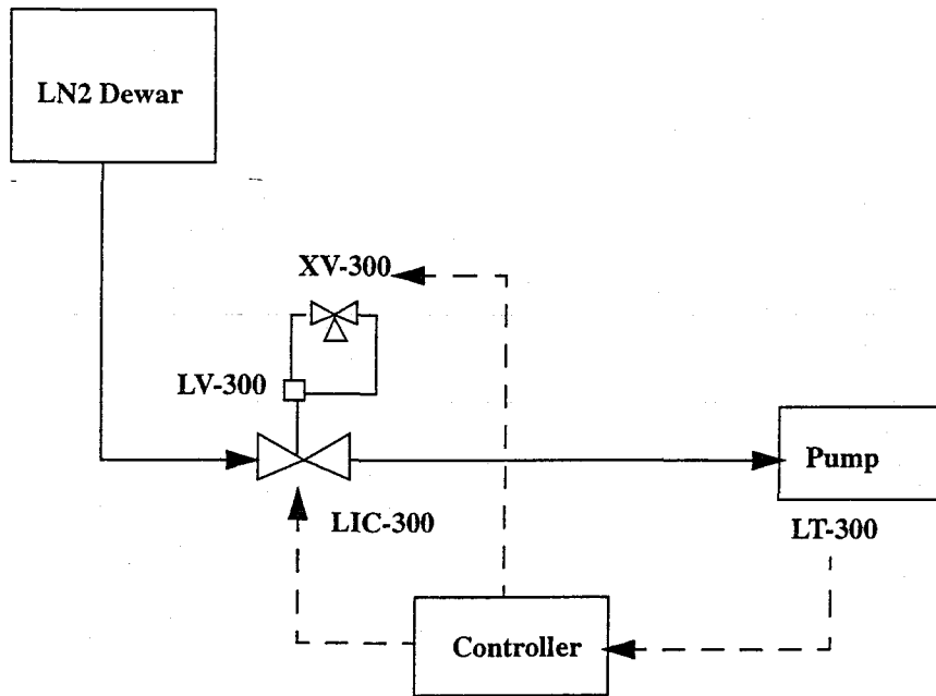
Figure 4: Cryopump Level Control Loop
