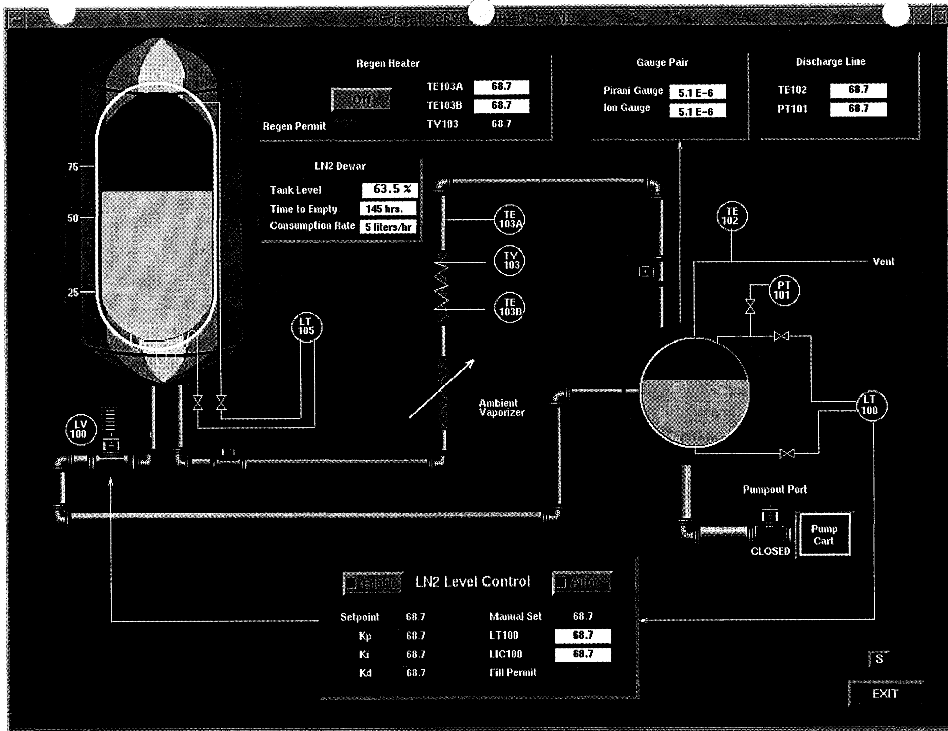
Figure 8: 80K Pump Detail Display
