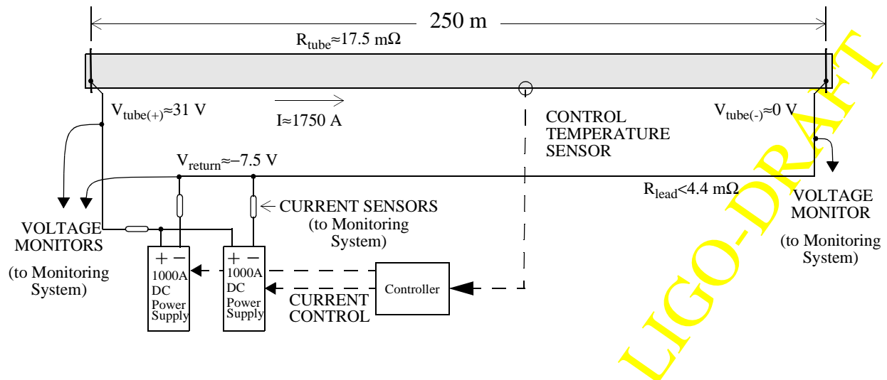
Figure 7: DC power supply control and connections to beam tube
