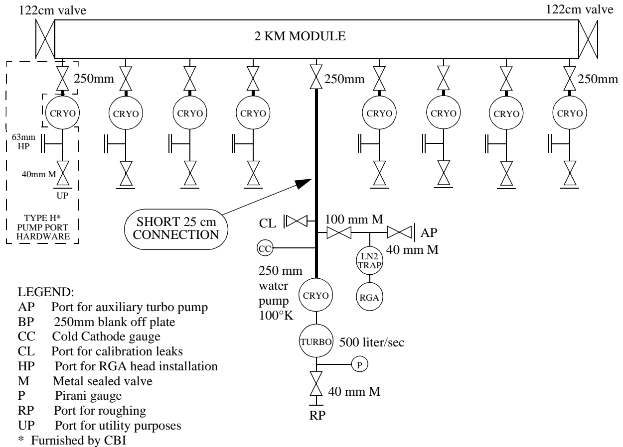
Figure 8: Schematic of vacuum pumps and RGA during bakeout
