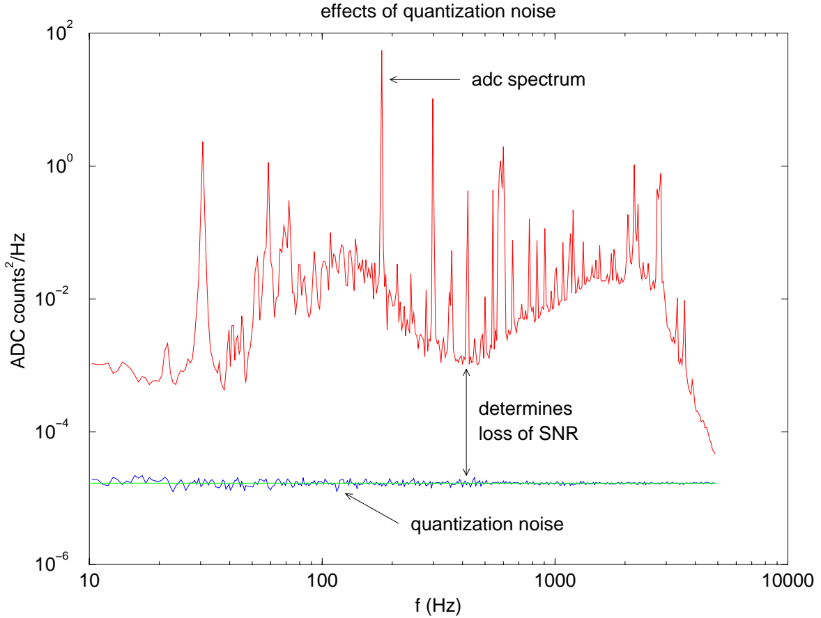
FIG. 1. The IFO power spectrum in (\text{ADC counts})^2/\text{Hz} is shown in red. This may be compared to the expected spectrum of quantization error \Delta^2/12f_N shown in green. The expected level of quantization noise was also simulated by replacing the IFO output with uniformly distributed random numbers on the interval (-\Delta/2, \Delta/2) , shown in blue. The ratio of the powers at the indicated point determines our upper bound on the fractional loss in signal to noise ratio.
