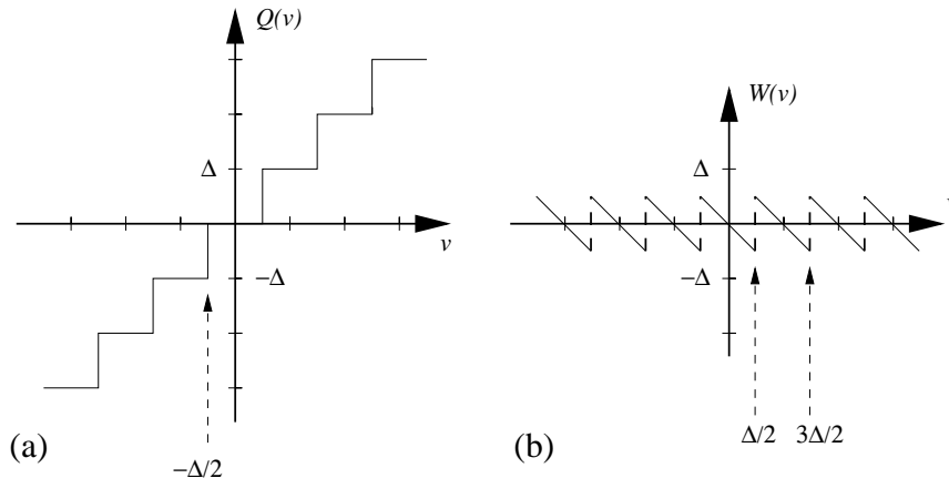
FIG. 2. (a) The quantization function Q(v) which maps the analog signal into integer multiples of \Delta , the quantization level, by rounding. (b) The error function which is defined as W(v) = Q(v) - v .
