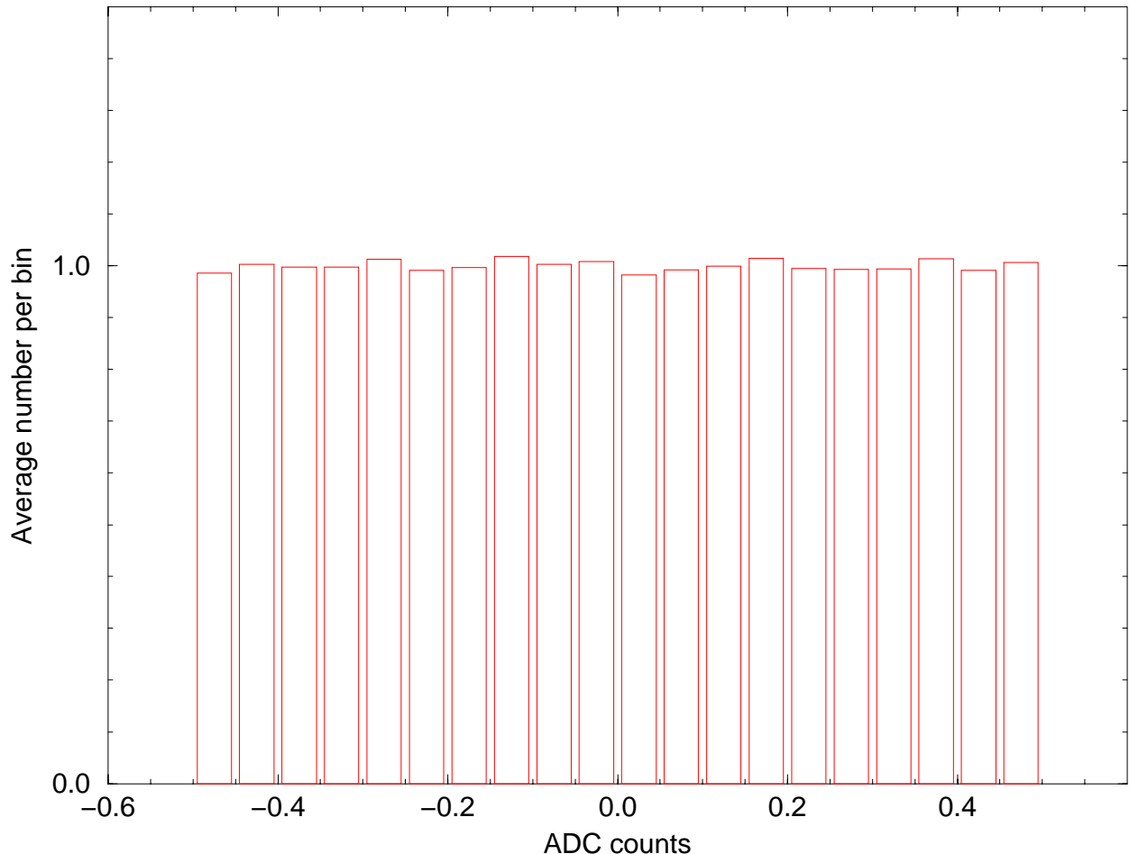
FIG. 4. Simulated Gaussian noise, with the power spectral density of the 40m prototype was quantized as describe above with \Delta = 1 . The quantization noise from 131072 samples was binned into 20 bins in the range (-0.5, 0.5] , and averaged (divided by 131072/20 ). The results shows that this noise is indeed uniformly distributed throughout the interval.
