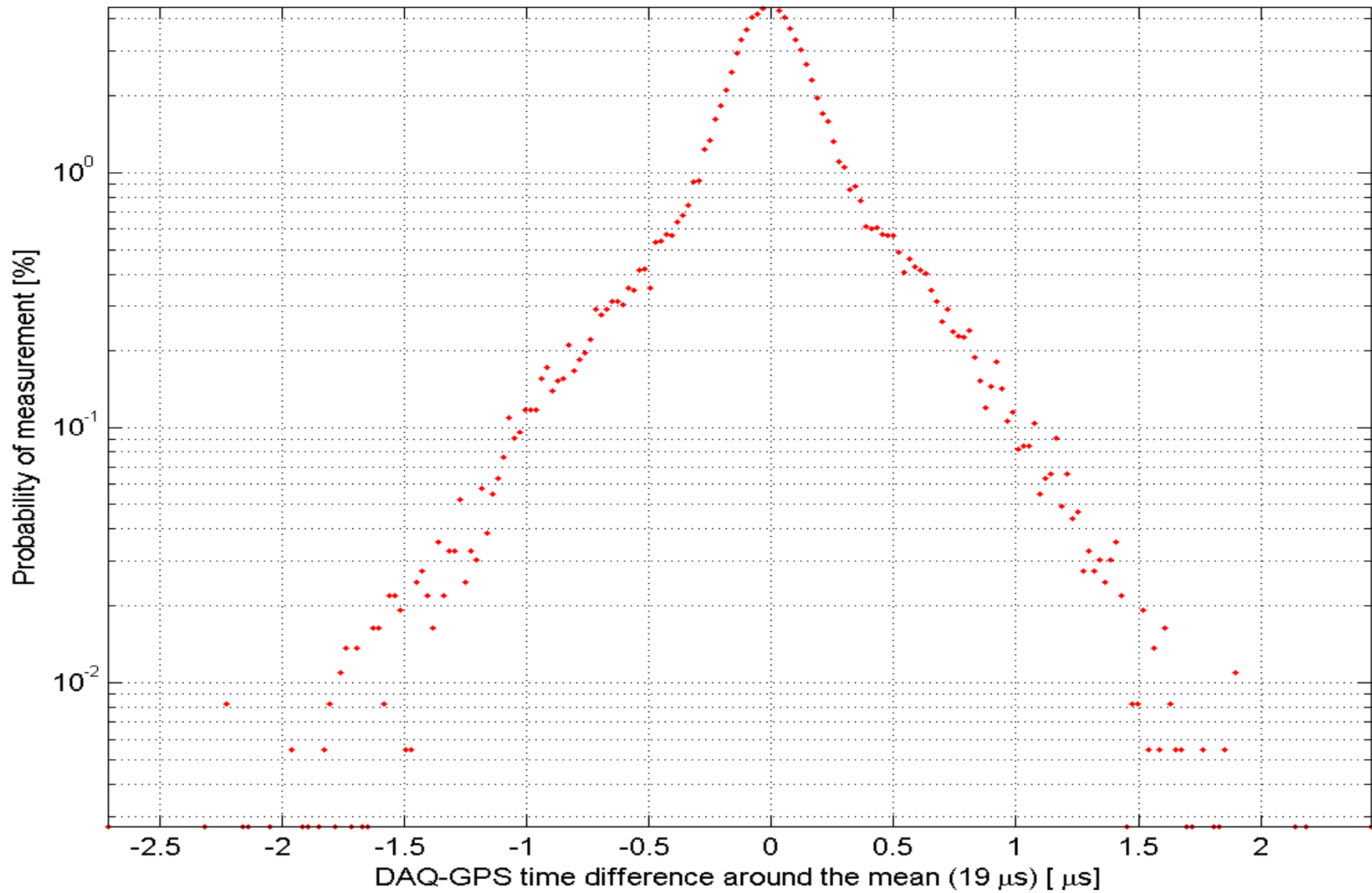
L1 EY timing performance during the S4 run
