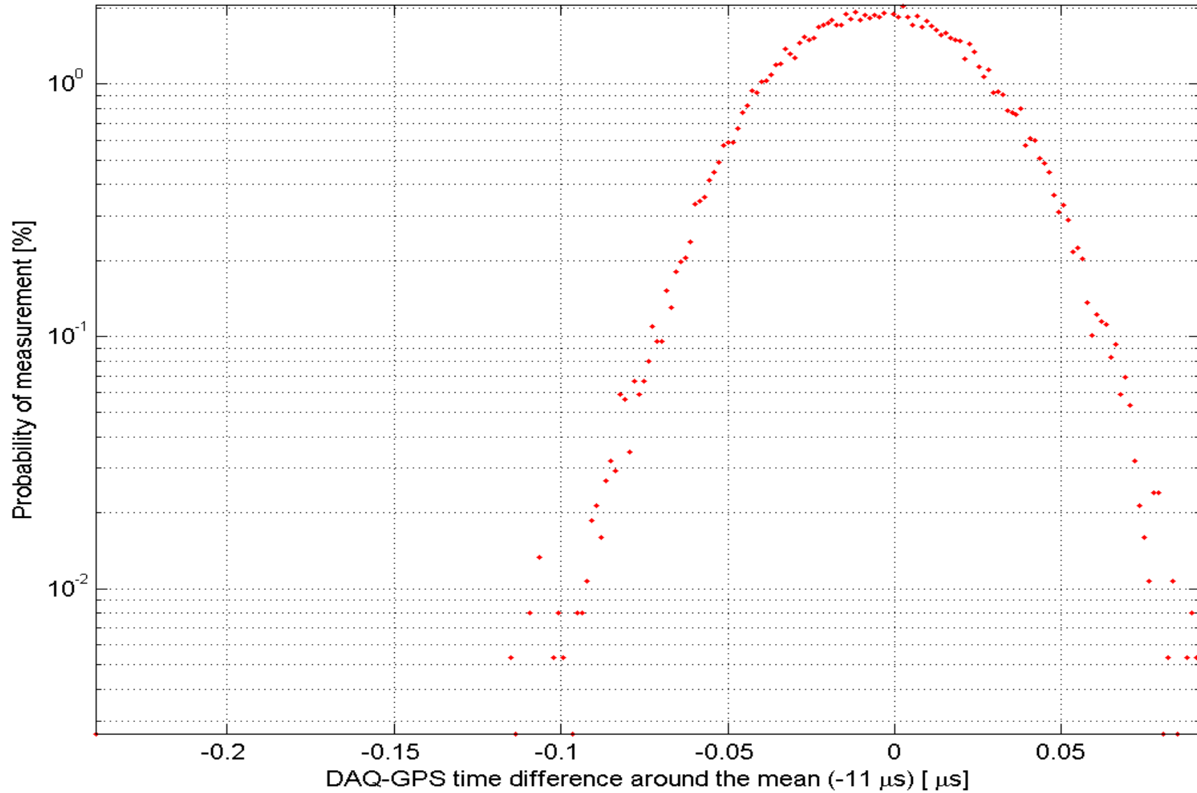
H2 AUX timing performance during the S4 run
