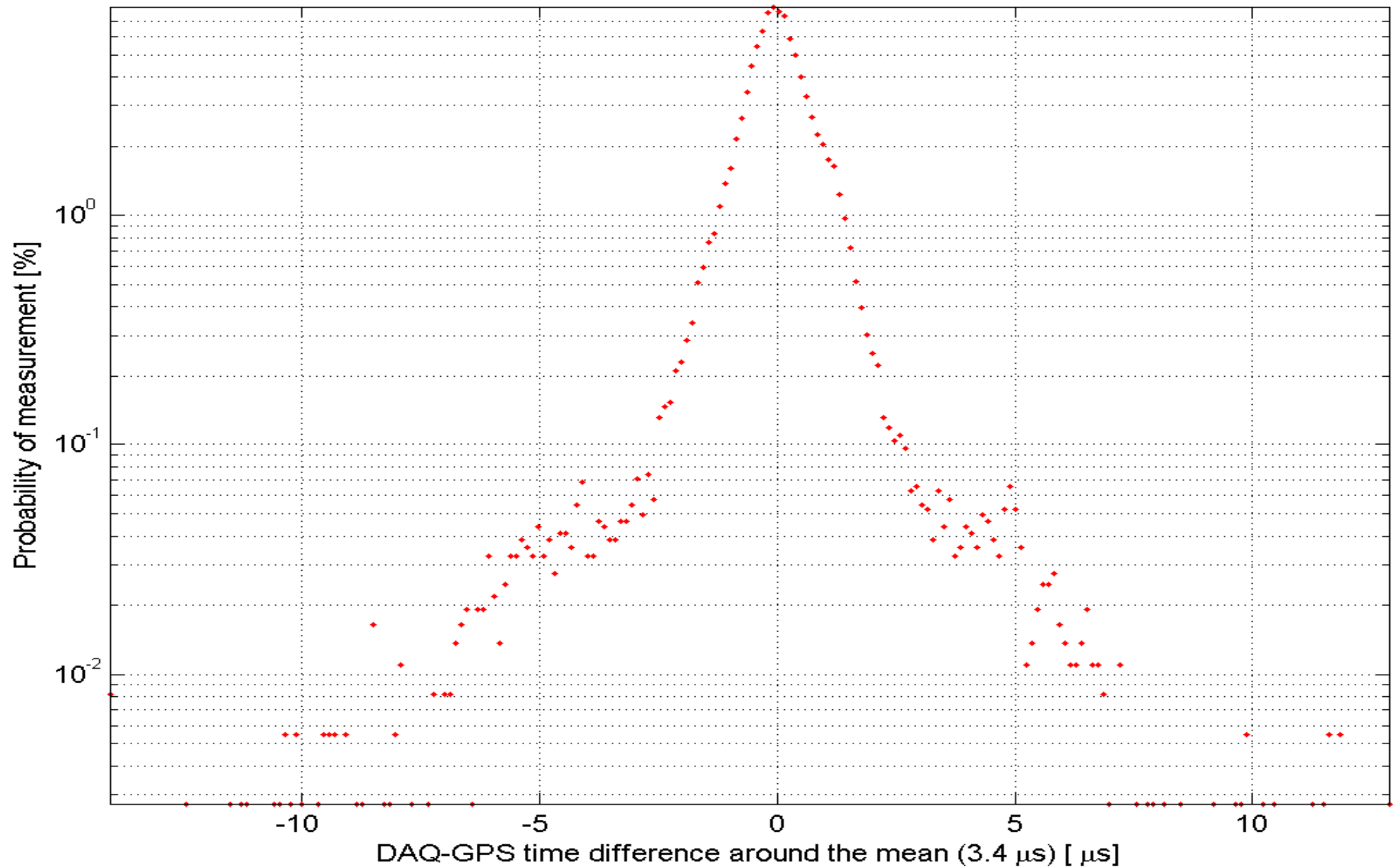
L1 LSC timing performance during the S4 run
