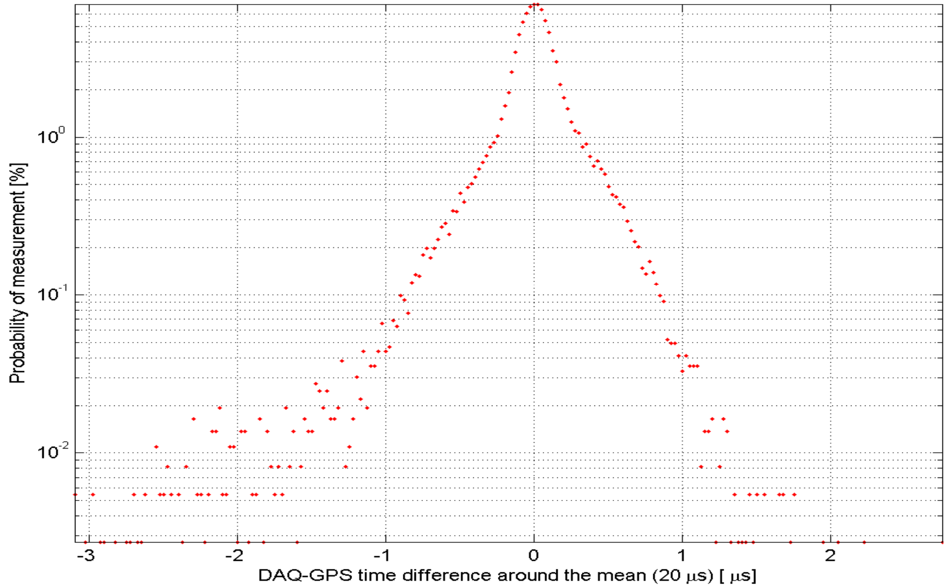
L1 PEM timing performance during the S4 run
