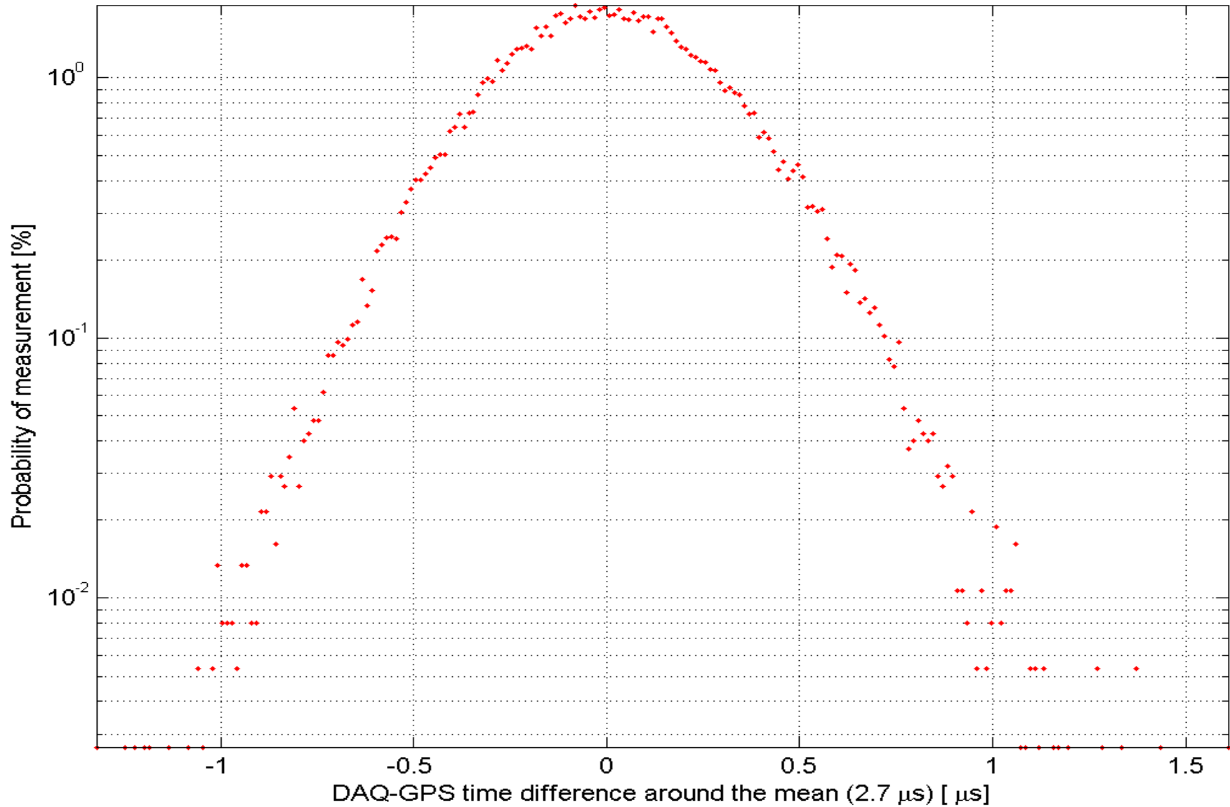
H1 LSC timing performance during the S4 run
