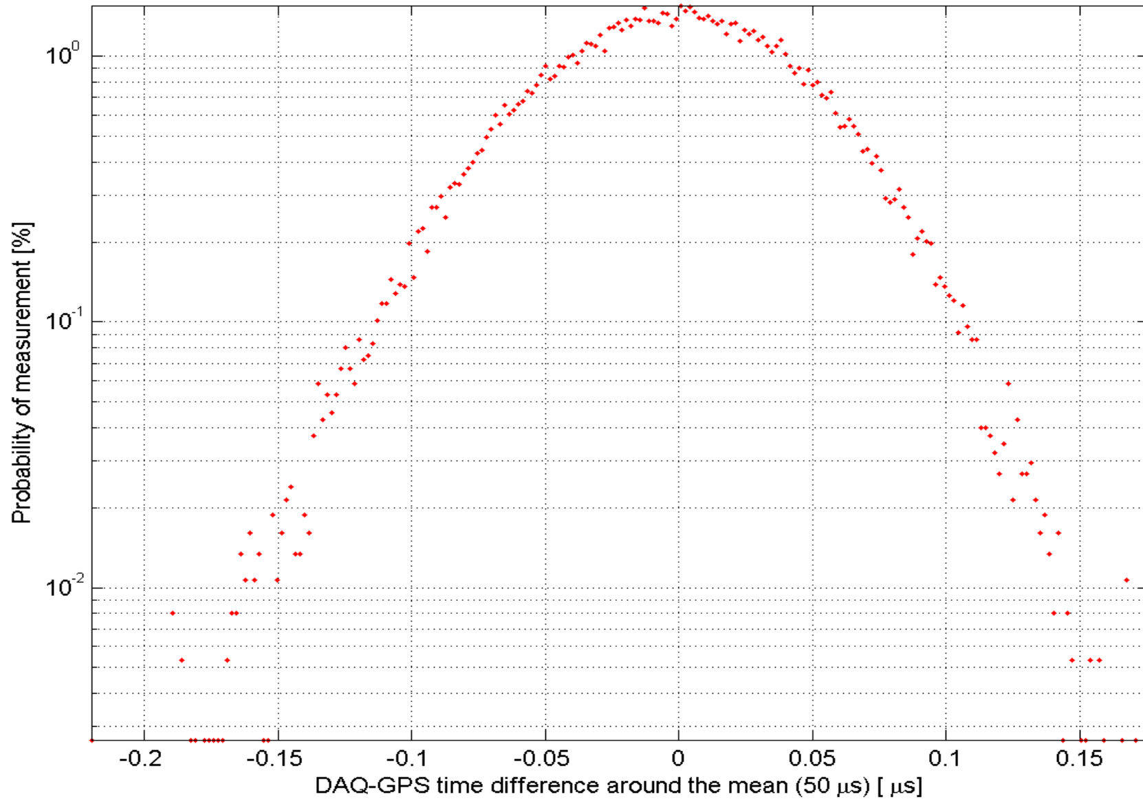
H1 EY timing performance during the S4 run
