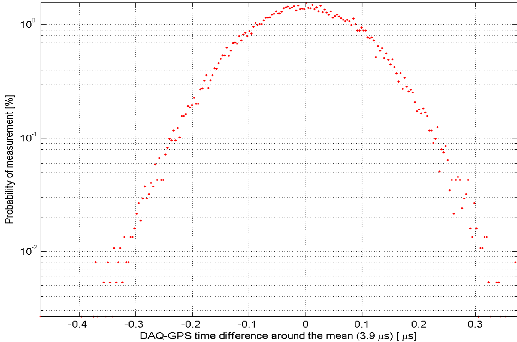
H2 LSC timing performance during the S4 run
