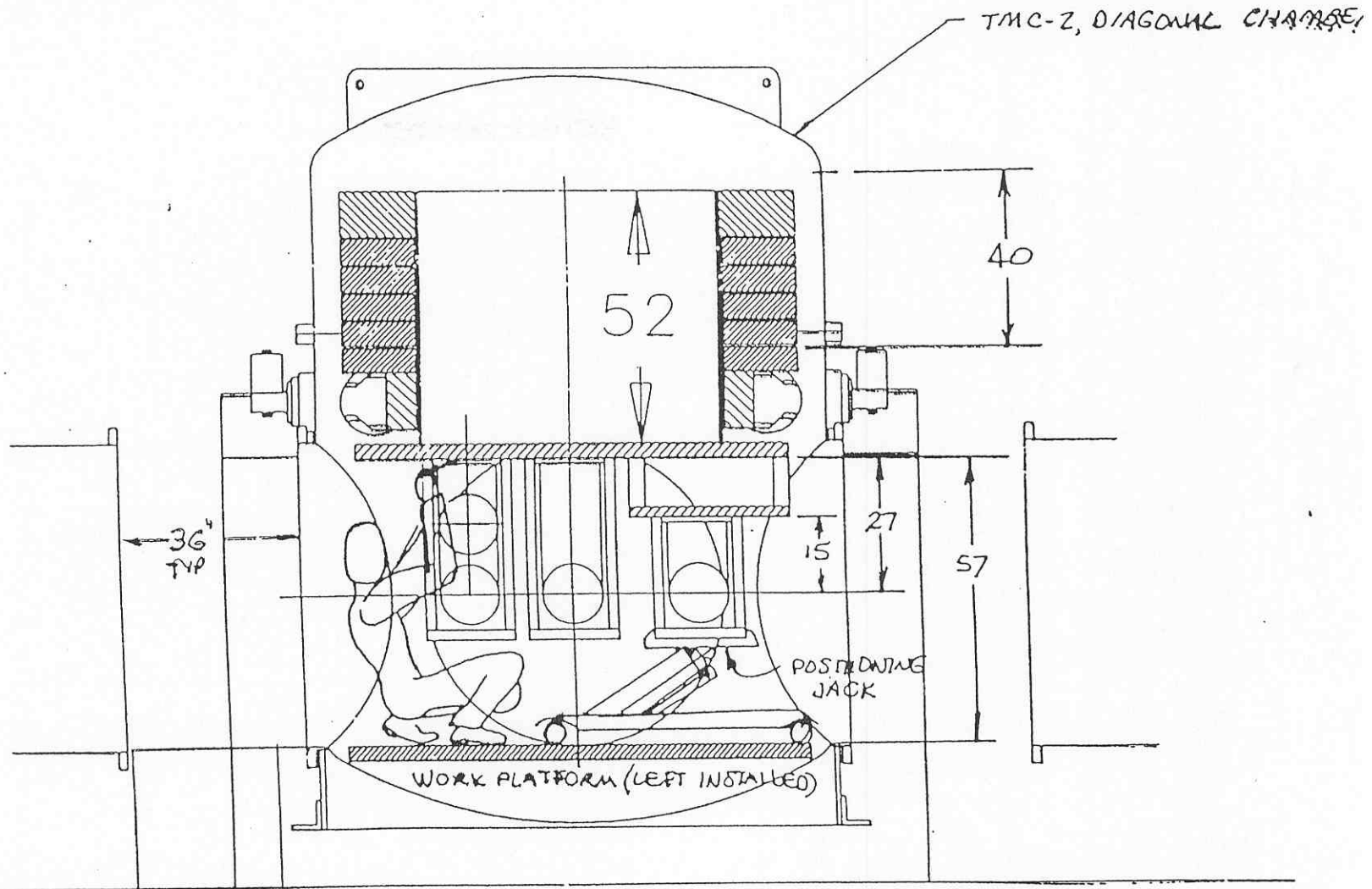
FIG. 3 INTERNAL ACCESS
