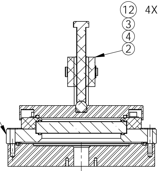
SECTION B-B (ROTATED 90 DEGREES)
