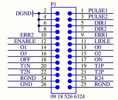
DB25/female
