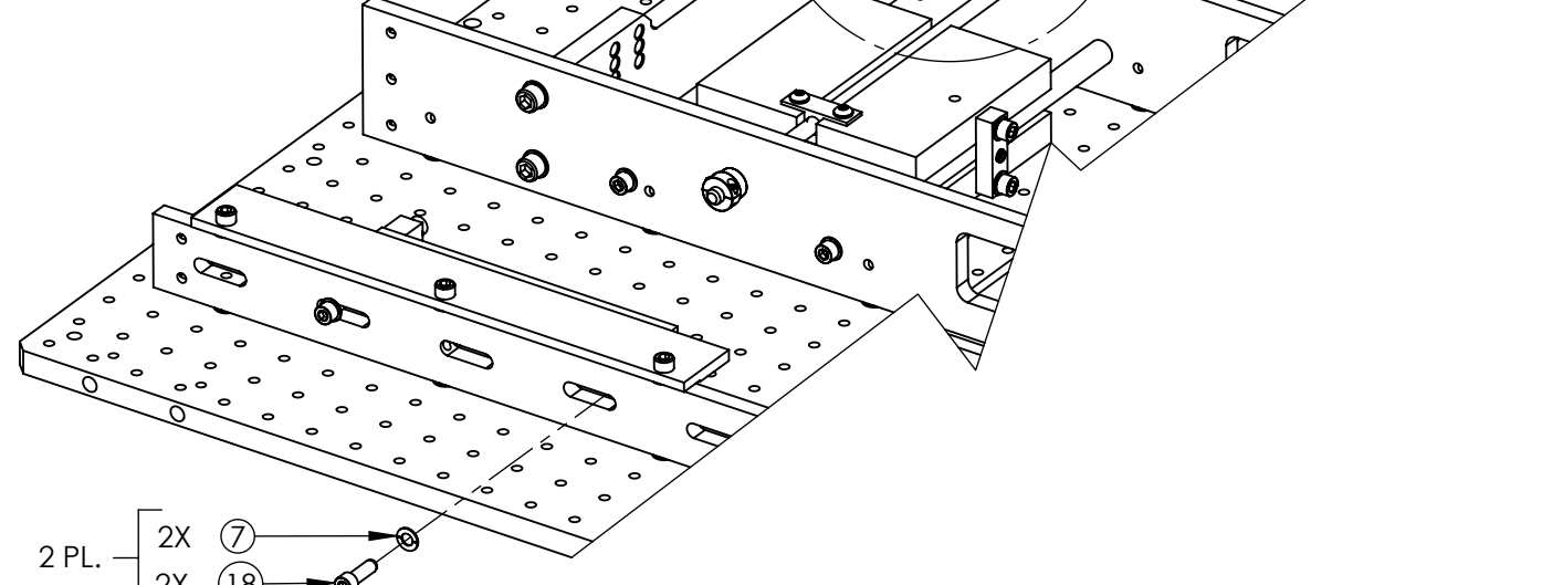
ASSY. STEP 4 (PARTIAL VIEW SHOWN)
