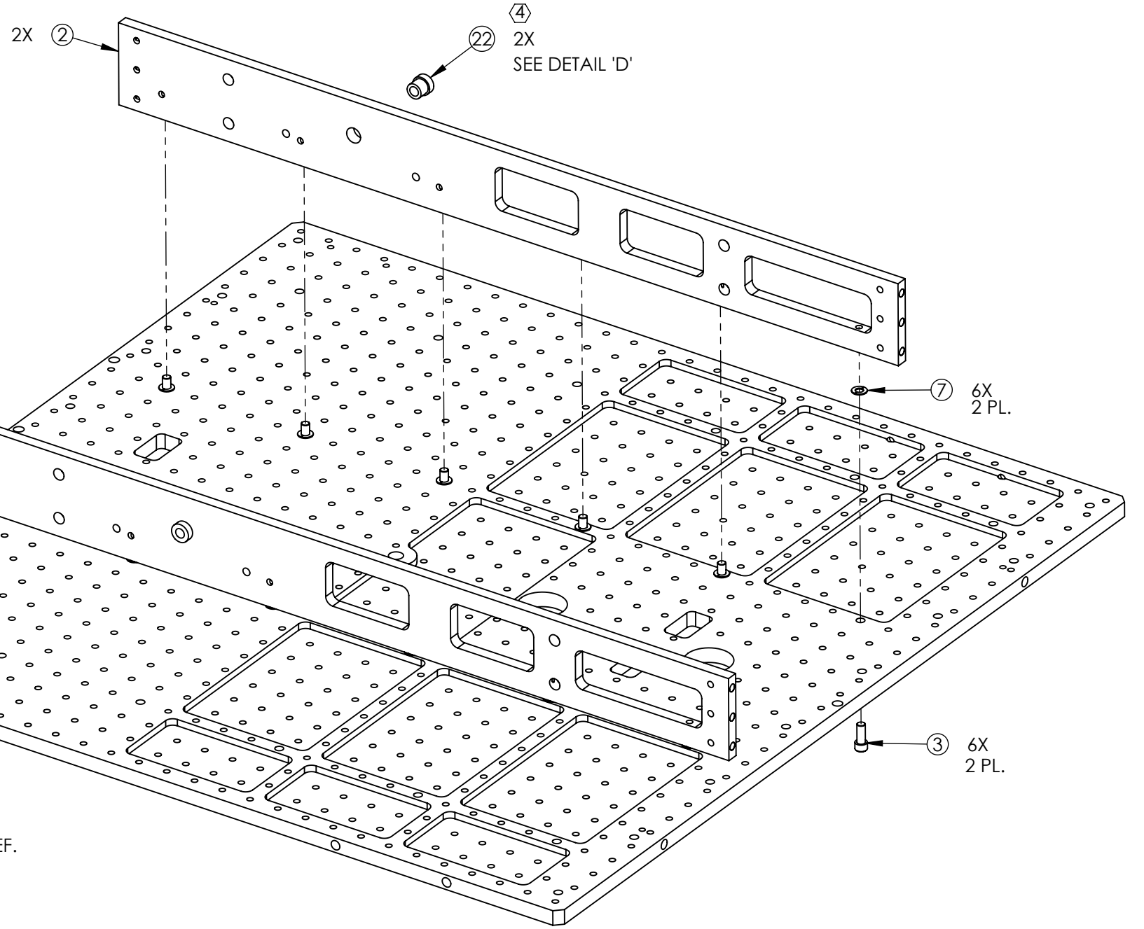
ASSY. STEP 1
