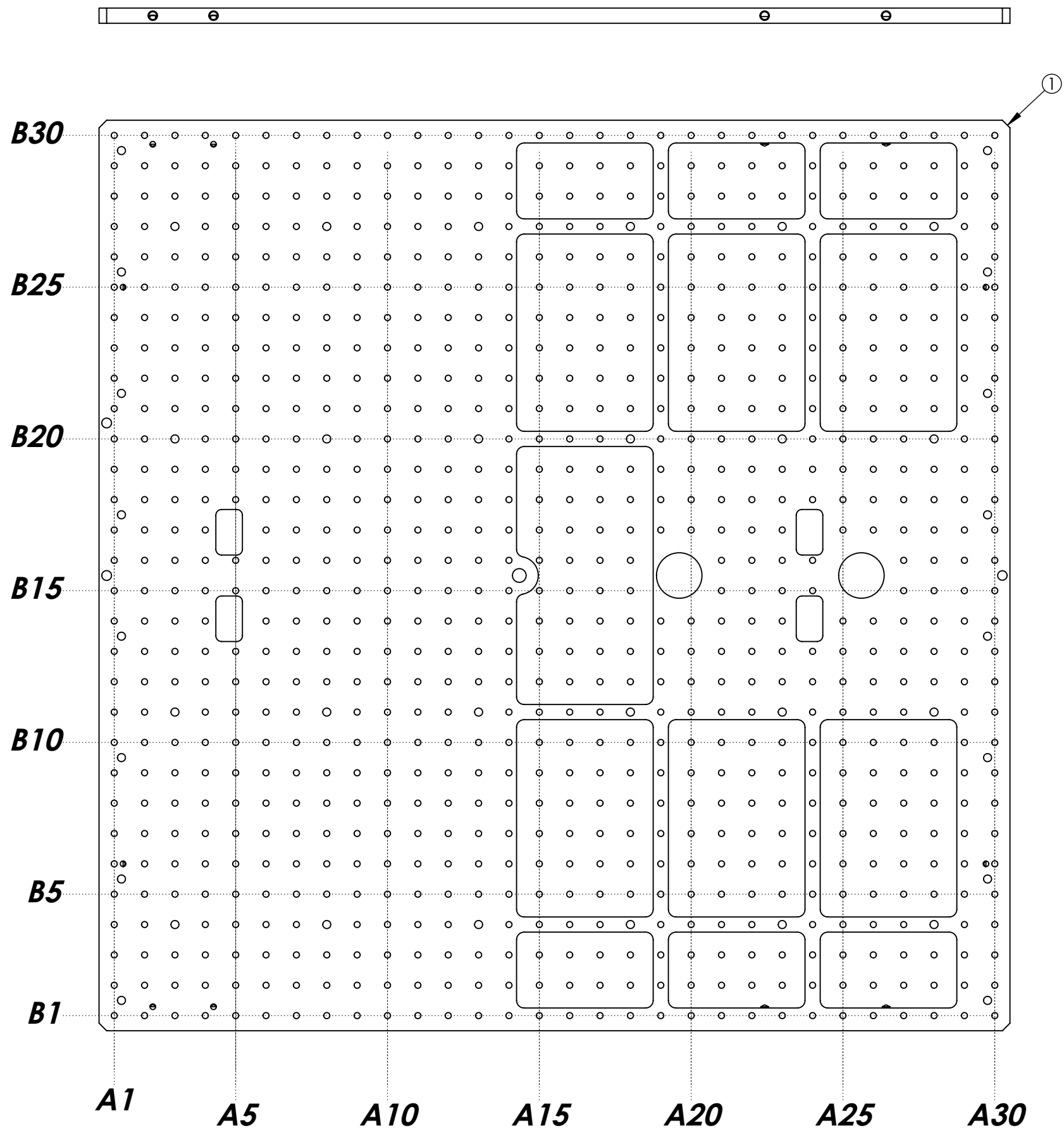
BOTTOM VIEW
