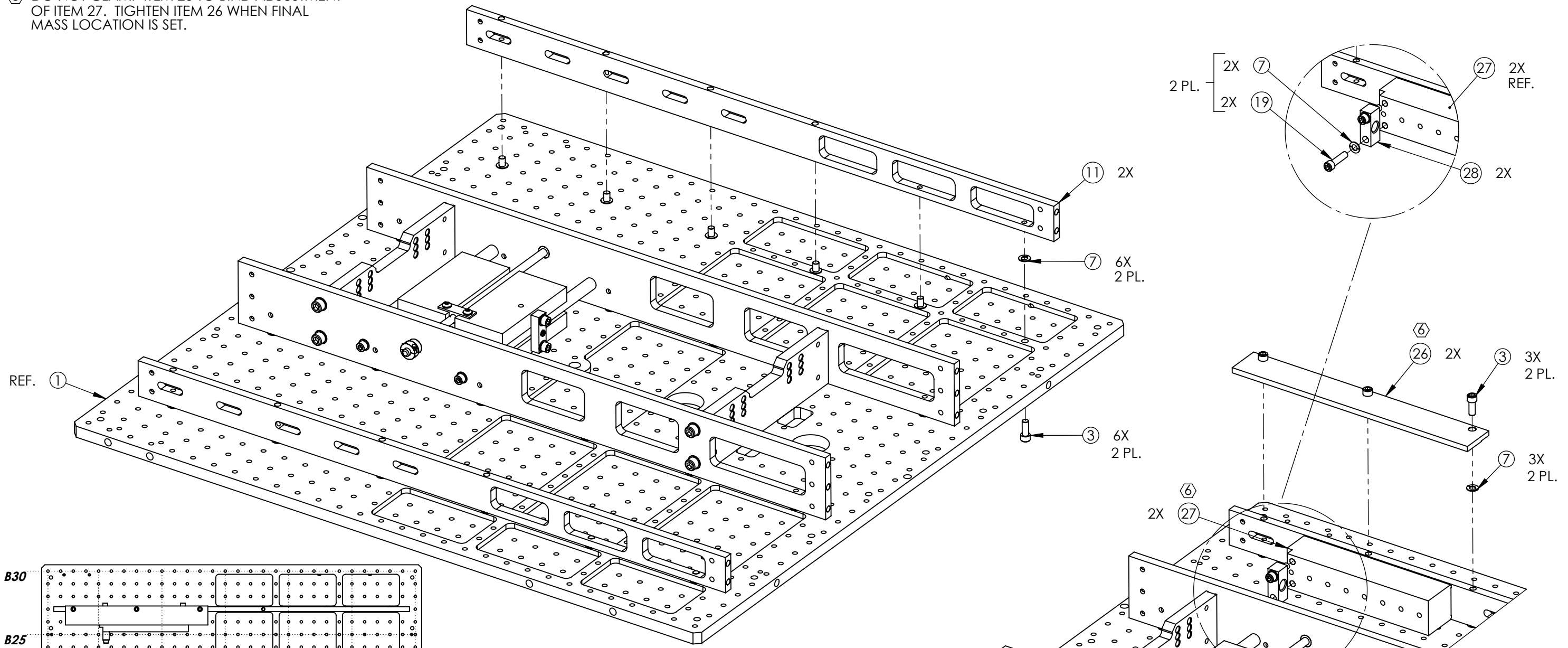
ASSY. STEP 3
