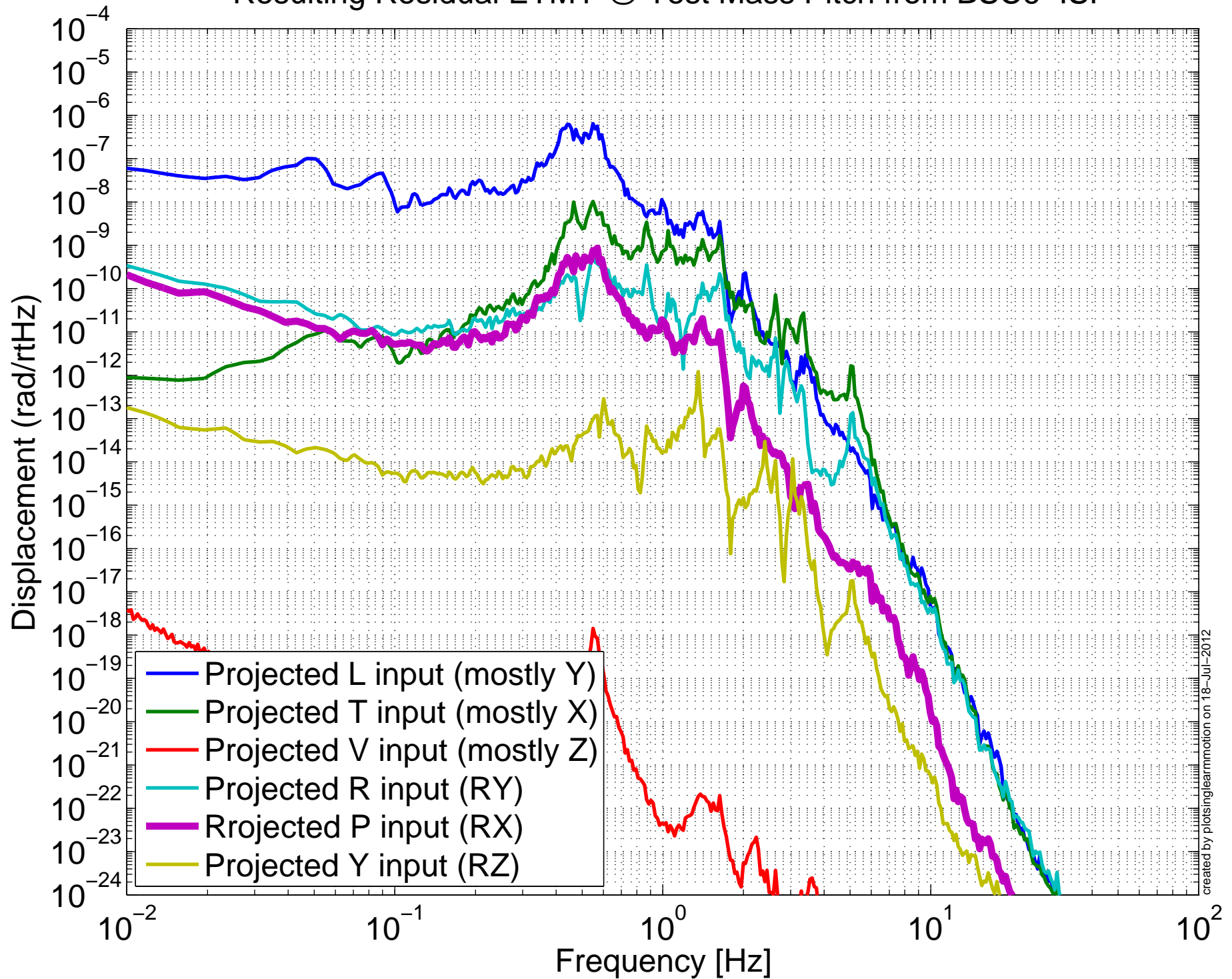
Resulting Residual ETMY @ Test Mass Pitch from BSC6-ISI
