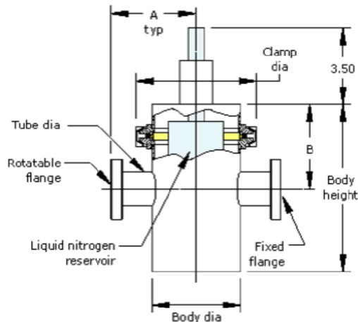
434016 - LiquidNitrogenTrap, 6"Body, 4.5"OD
