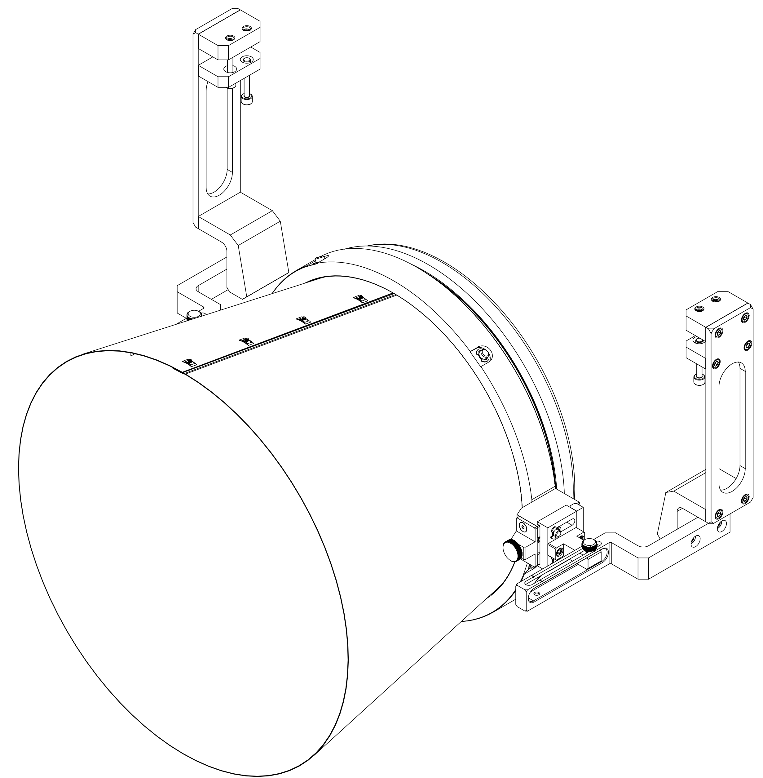
ISO VIEW
