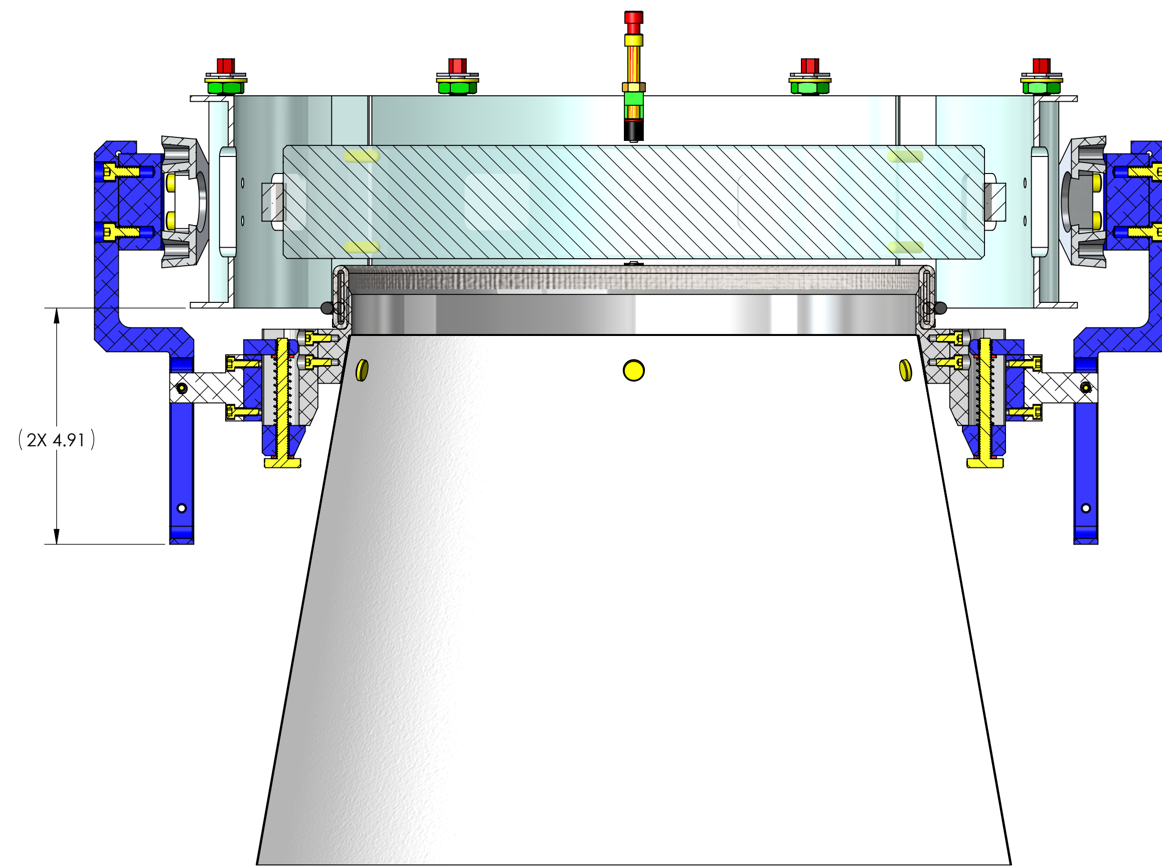
SECTION C-C
