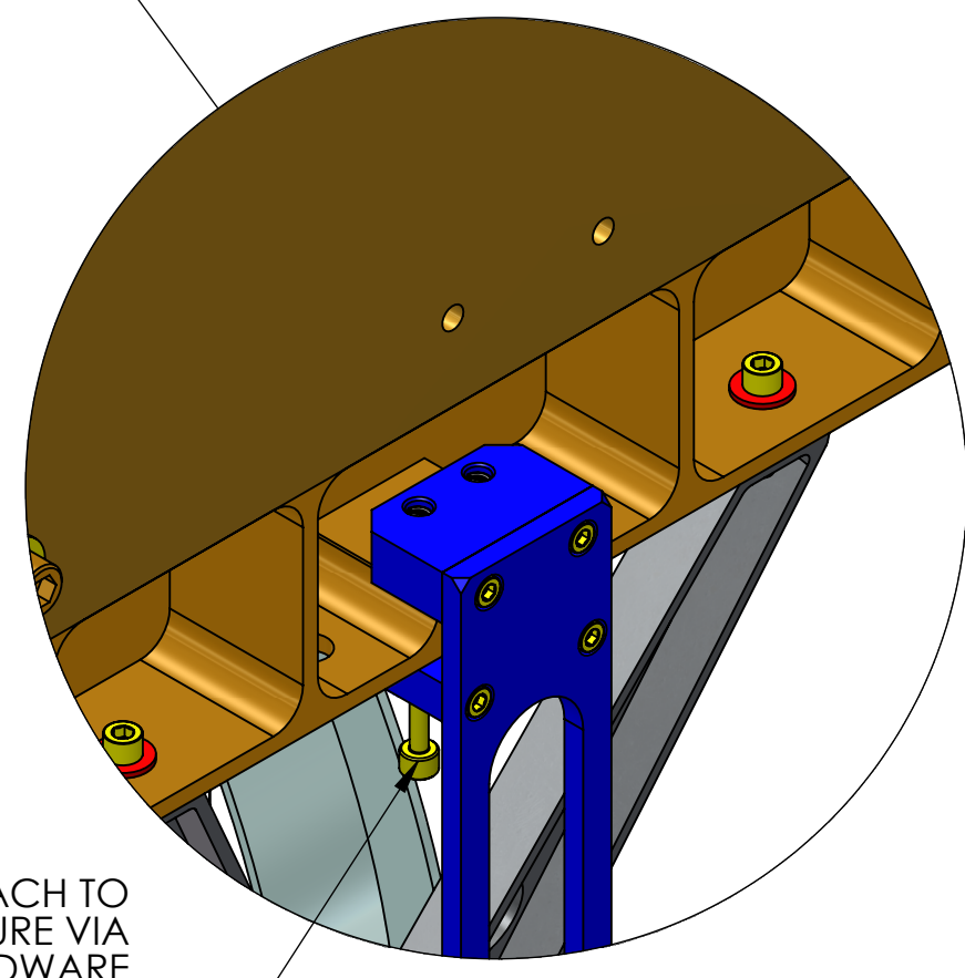
DETAIL B
