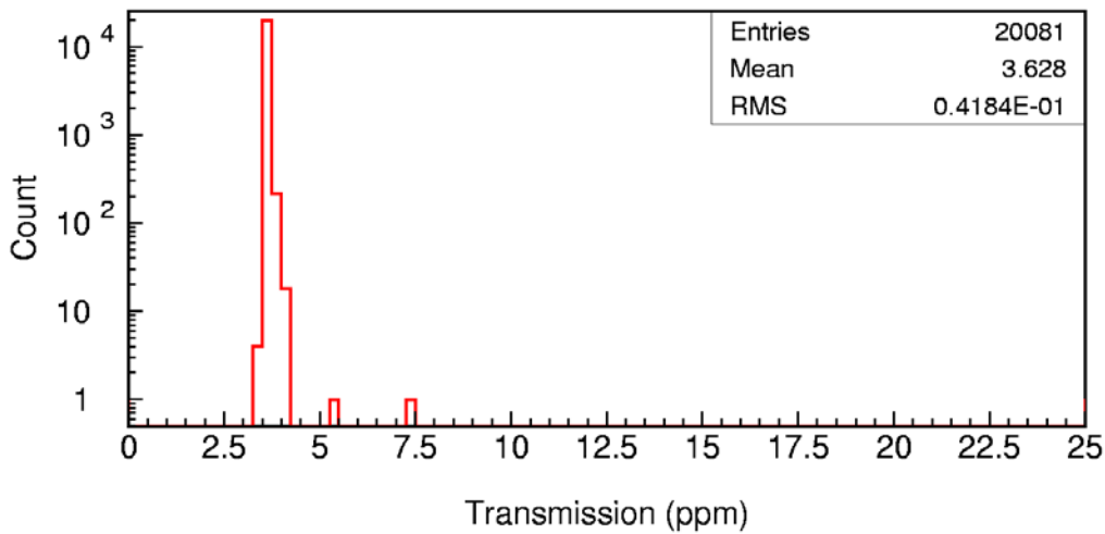
Fig. 1 ETM12 transmission over a 160 mm diameter aperture.
