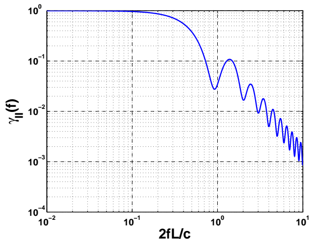
FIG. 4: A plot of the transfer function \mathcal{R}_I(f) = \gamma_{II}(f) normalized to unity for the strain response of an equal-arm Michelson interferometer. The dips in the transfer function occur around integer multiples of c/(2L) , where L is the arm length of the interferometer.
