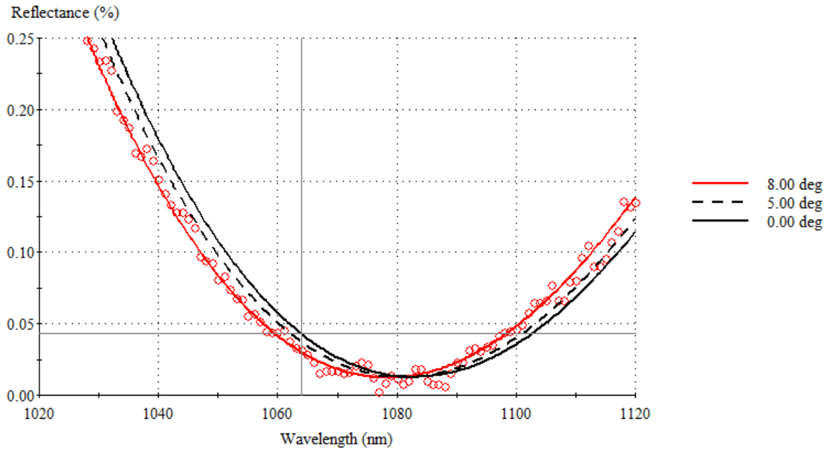
Reflectance, P-1592 Fitted data at 8deg (red) Modeled at 0deg and 5deg (black)
