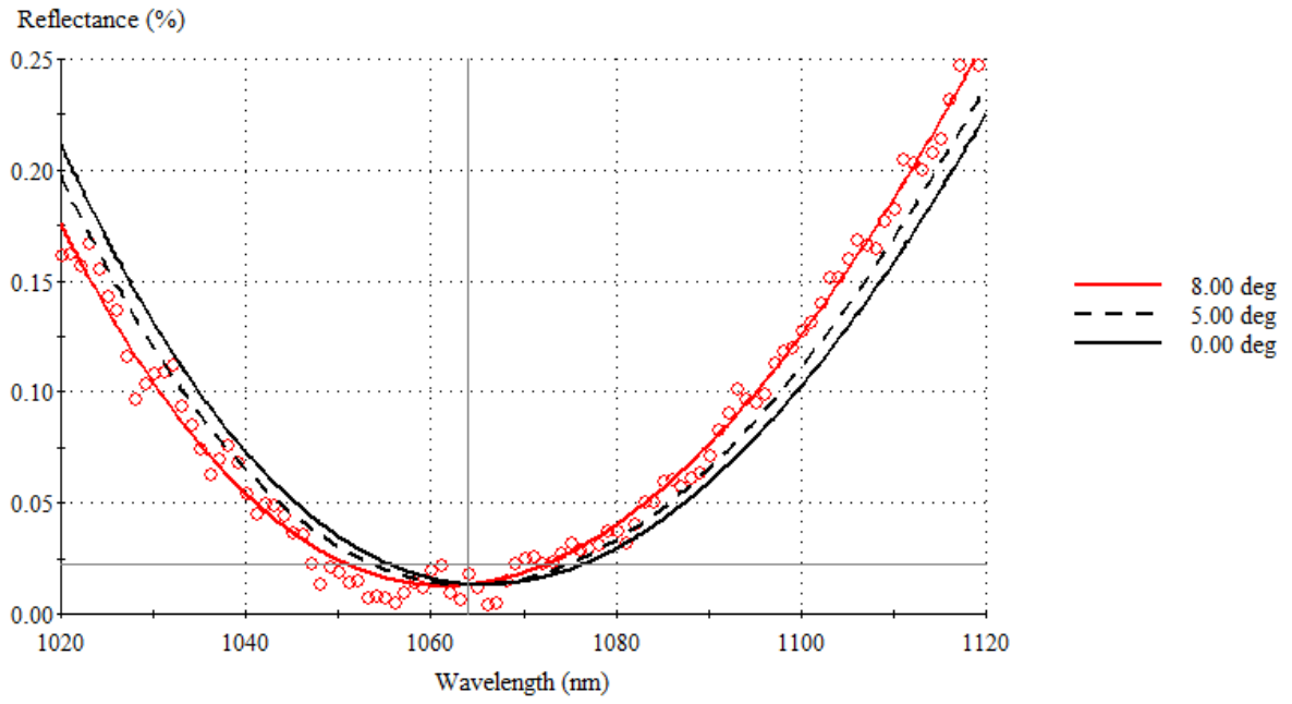
Reflectance, P-1593 Fitted data at 8deg (red) Modeled at 0deg and 5deg (black)
