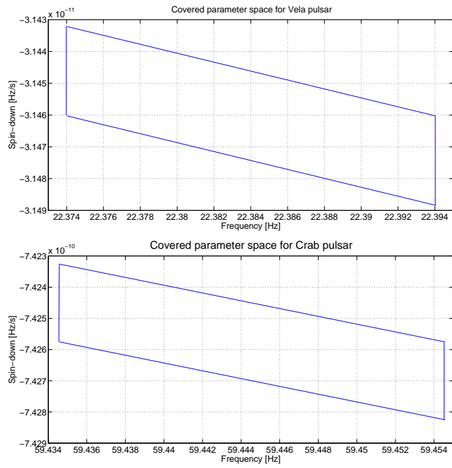
FIG. 4. The parallelograms delimit the portion of the f - \dot{f} plane covered in the narrow-band search for the Vela (upper plot) and Crab (bottom plot) pulsars. Only one value of \dot{f} has been considered in the analysis. The total number of points is given in the last column of Tab. II.
