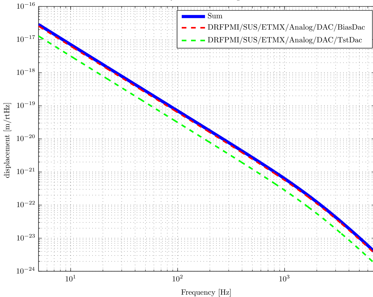
QUAD L3 NoiseBudget
