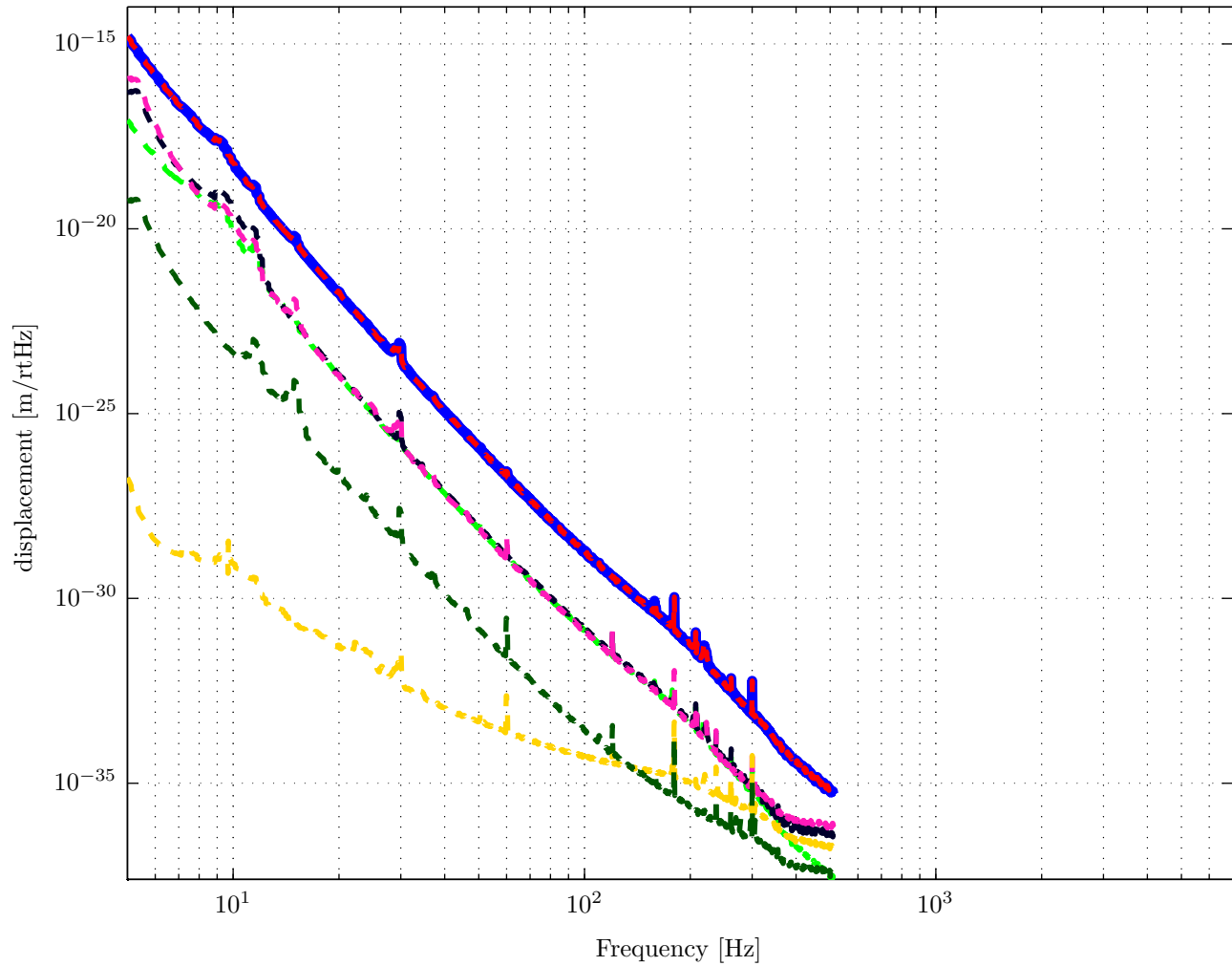
ITMX NoiseBudget
