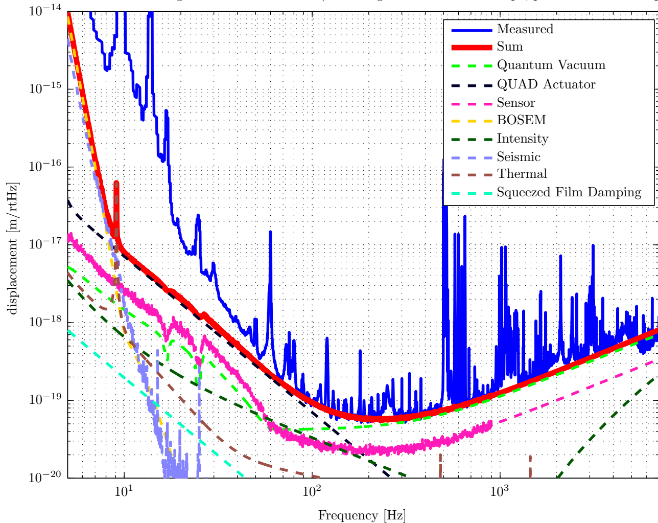
L1 DARM NoiseBudget at GPS 1091861260 (BNS range observed 21.4816 Mpc, predicted 25.5952 Mpc)
