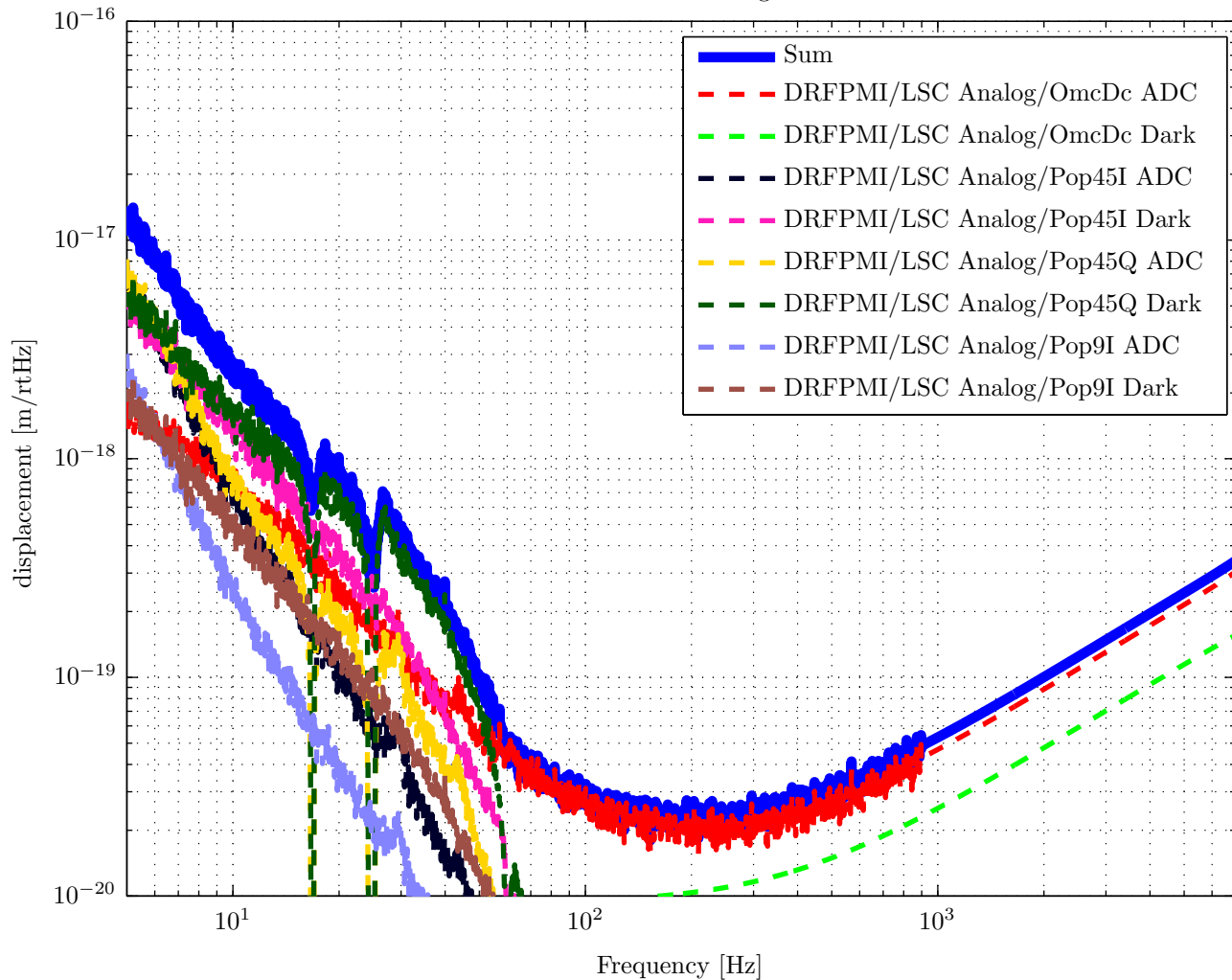
Sensor NoiseBudget
