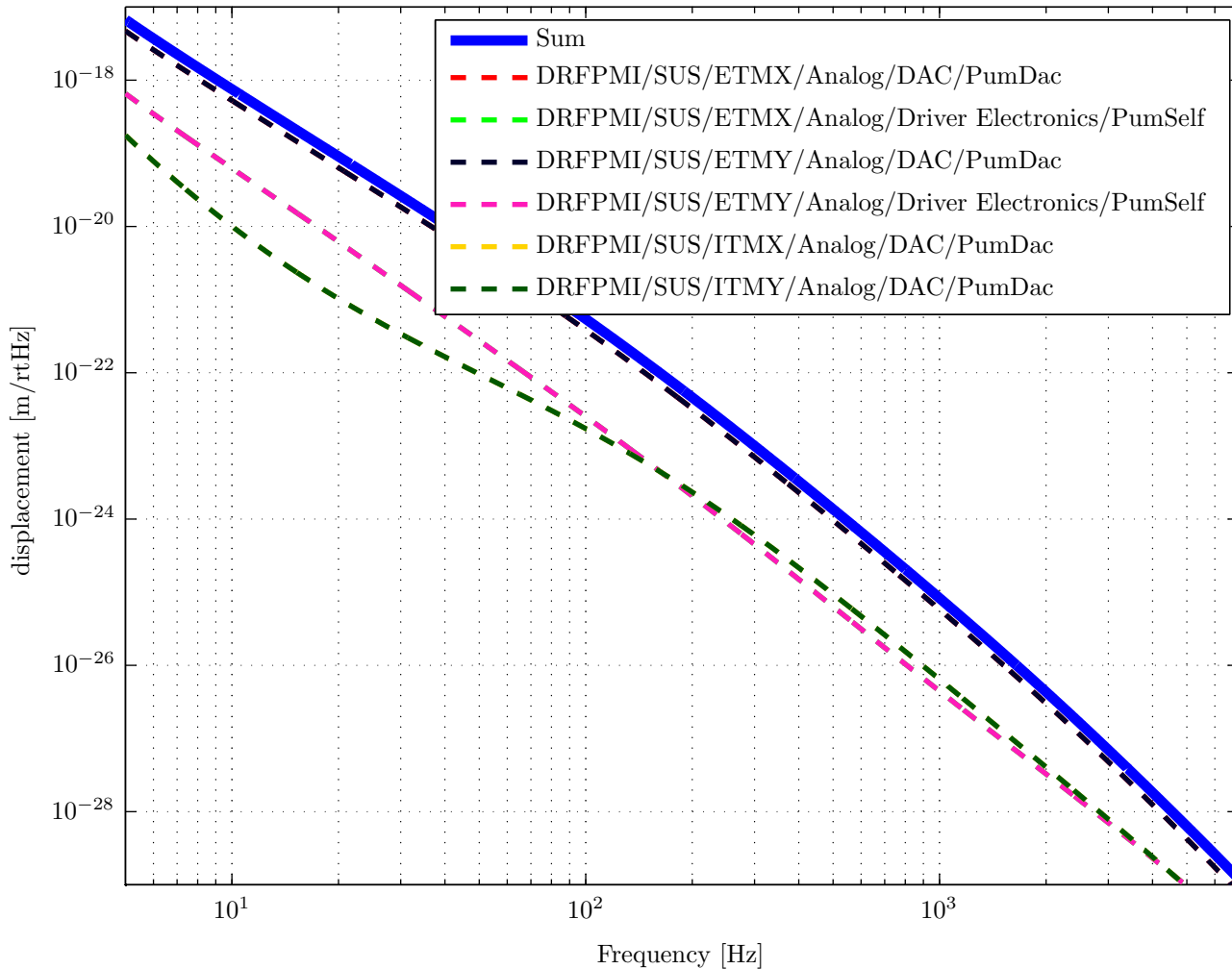
QUAD L2 NoiseBudget
