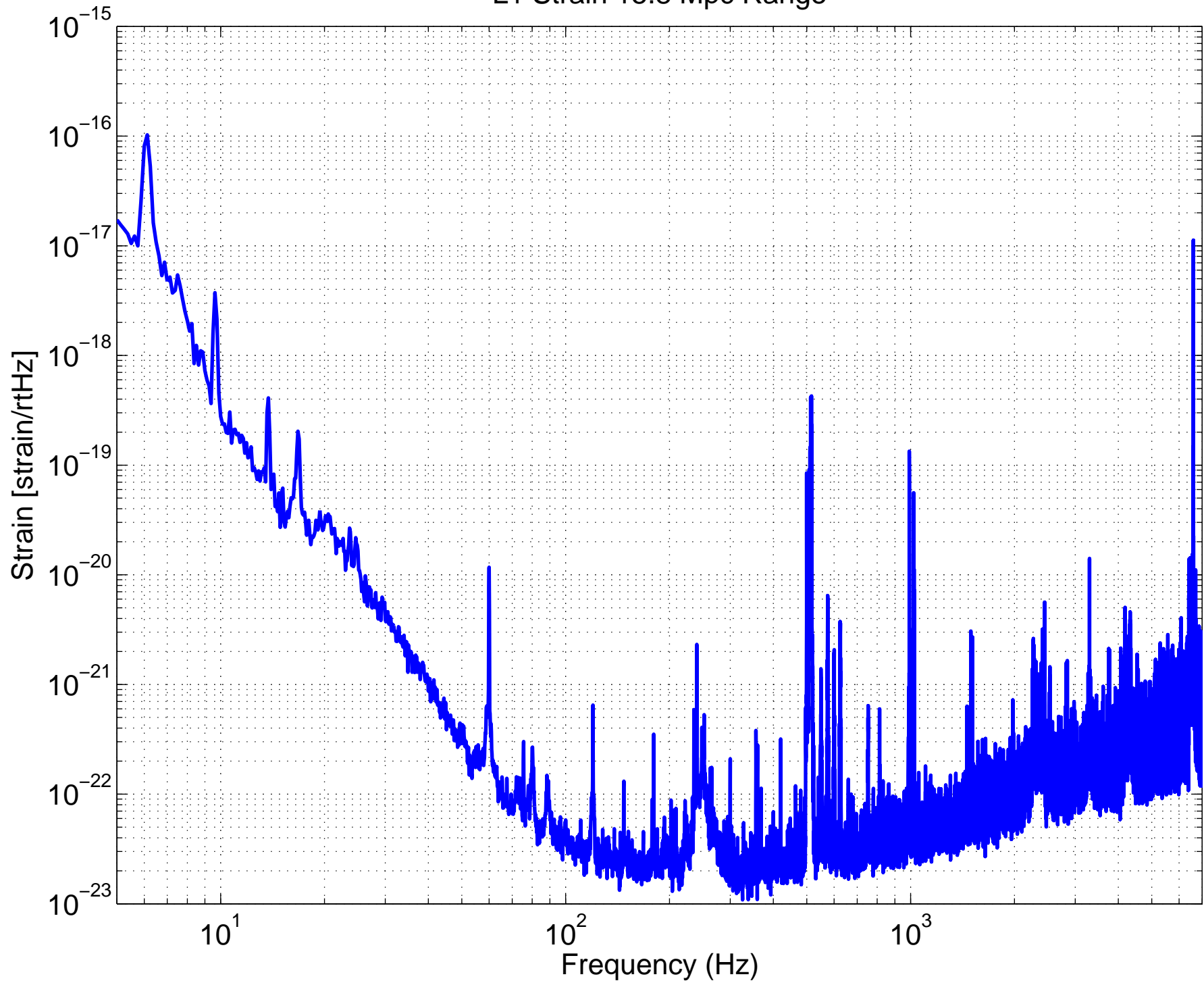
L1 Strain 15.8 Mpc Range
