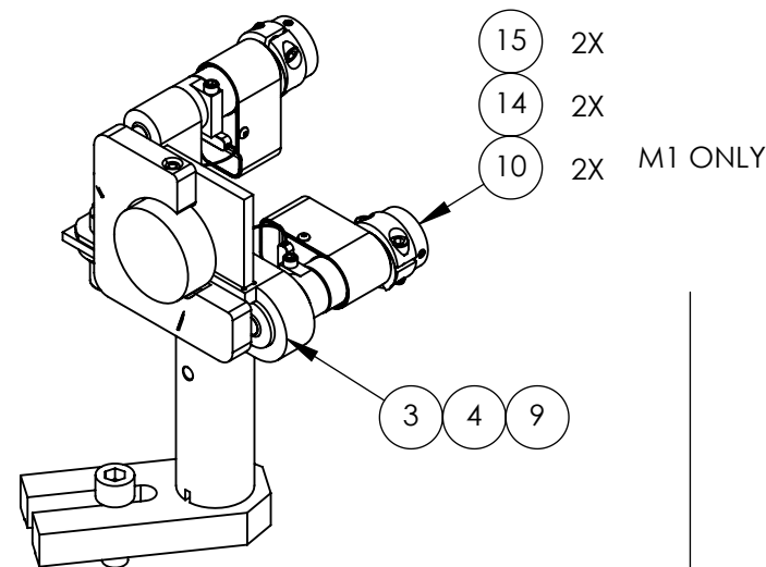
-01 DETAIL ISO VIEW, RIGHT SIDE (OFI M1 SHOWN)
