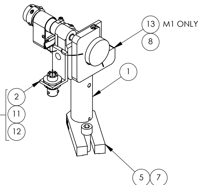
-01 DETAIL ISO VIEW, LEFT SIDE (OFI M1 SHOWN)
