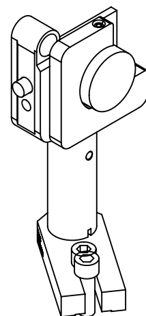
-02 DETAIL ISO VIEW, LEFT SIDE (OFI M2 SHOWN)
