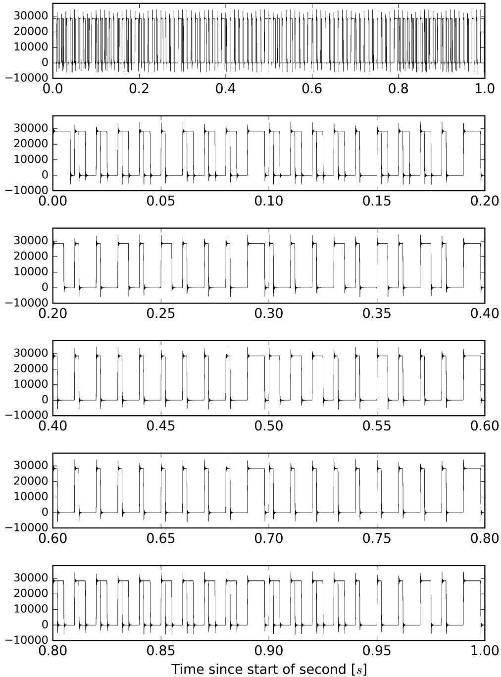
Overlay of L1:CAL-PCALY_IRIGB_OUT_DQ from 1172259768 to 1172259769
