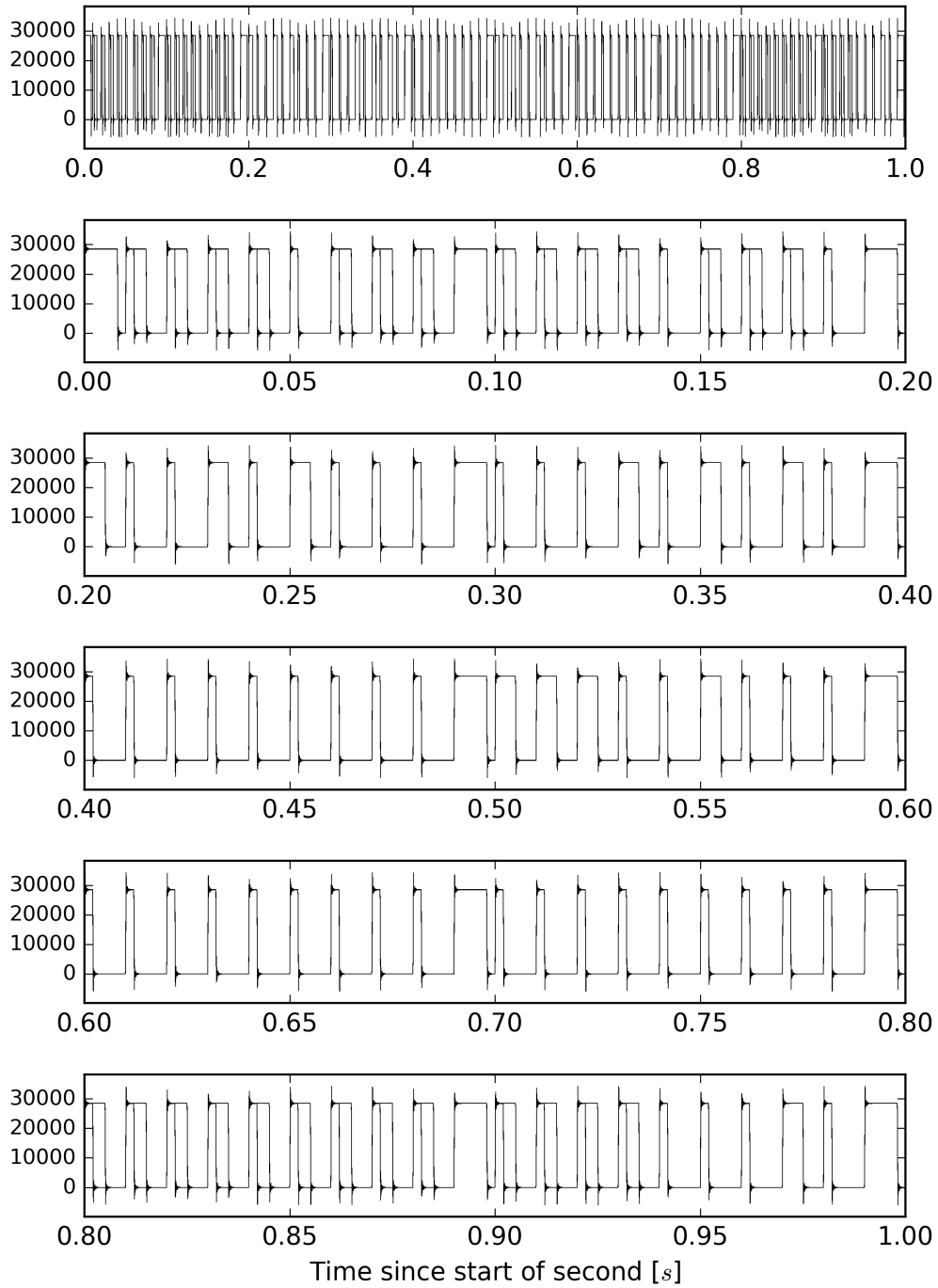
Overlay of L1:CAL-PCALX_IRIGB_OUT_DQ from 1172259768 to 1172259769
