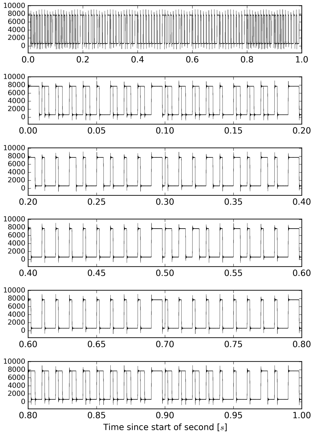
Overlay of H1:CAL-PCALX_IRIGB_OUT_DQ from 1172259768 to 1172259769
