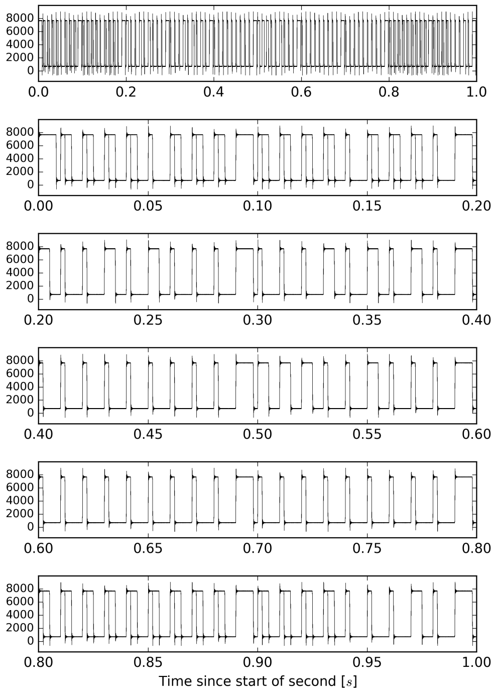
Overlay of H1:CAL-PCALY_IRIGB_OUT_DQ from 1172259768 to 1172259769
