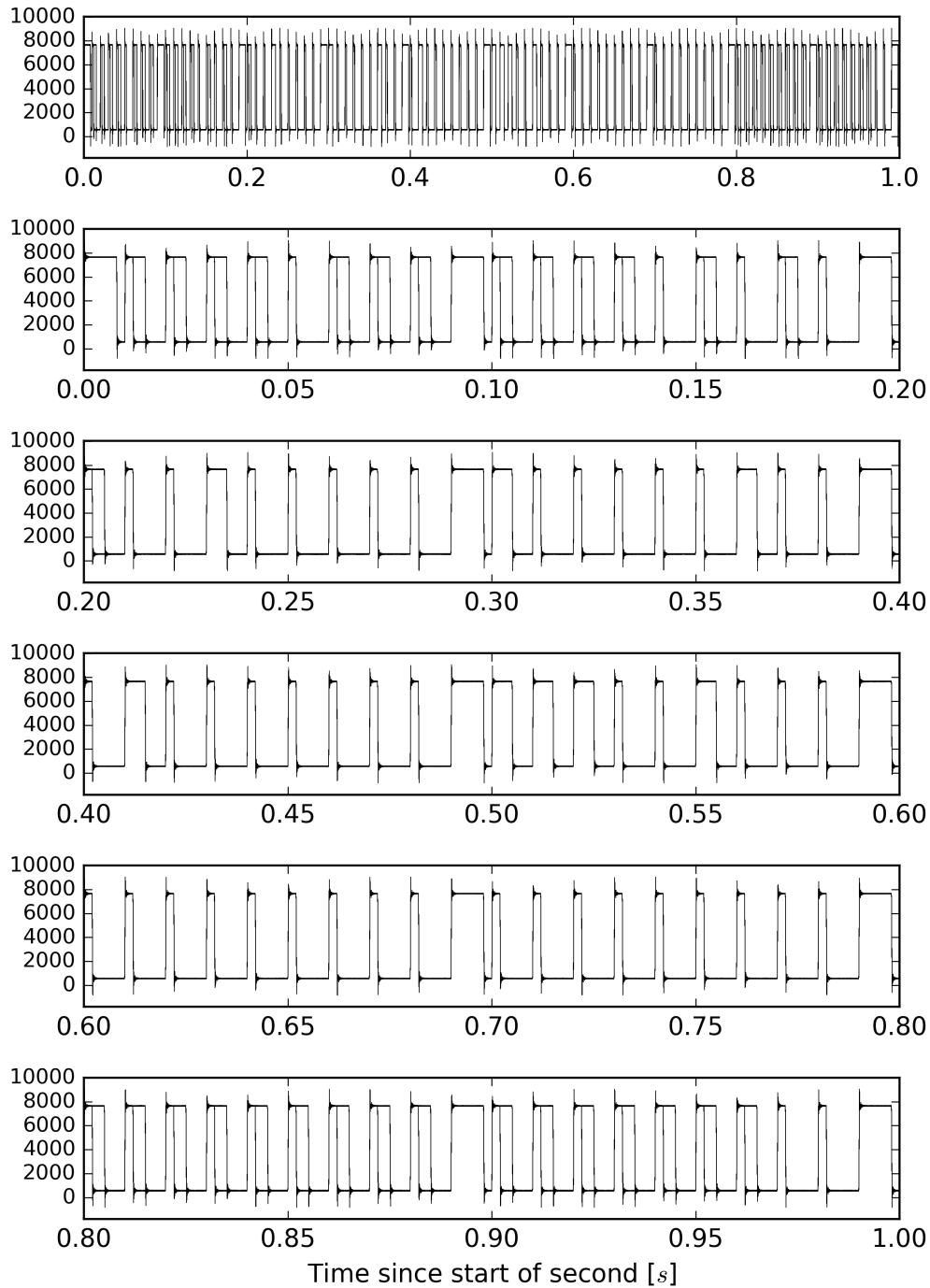
Overlay of H1:CAL-PCALX_IRIGB_OUT_DQ from 1186305218 to 1186305219
