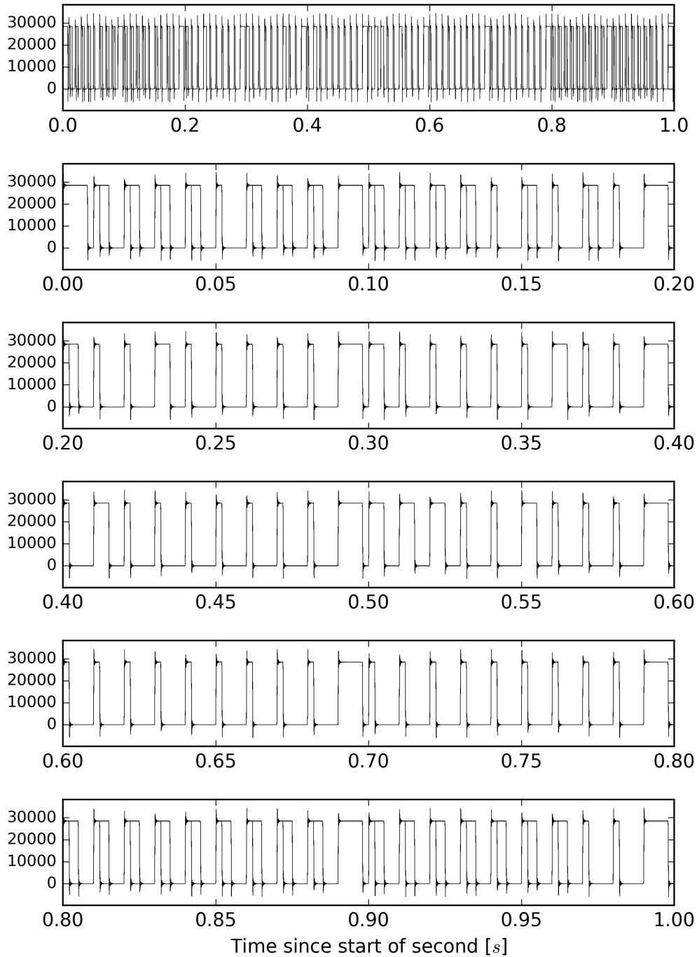
Overlay of L1:CAL-PCALX_IRIGB_OUT_DQ from 1186305218 to 1186305219
