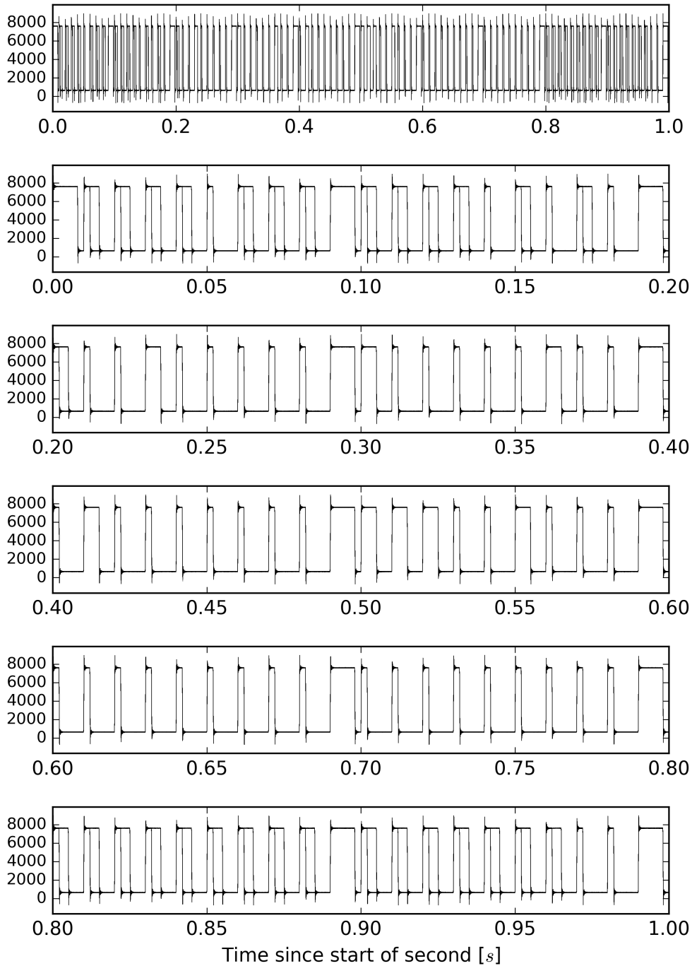
Overlay of H1:CAL-PCALY_IRIGB_OUT_DQ from 1186305218 to 1186305219
