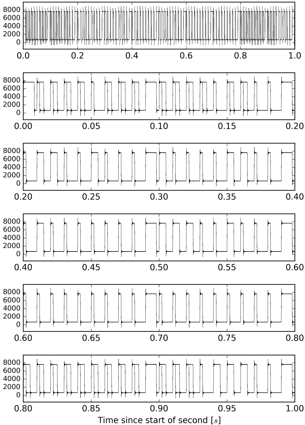
Overlay of H1:CAL-PCALY_IRIGB_OUT_DQ from 1187195763 to 1187195764
