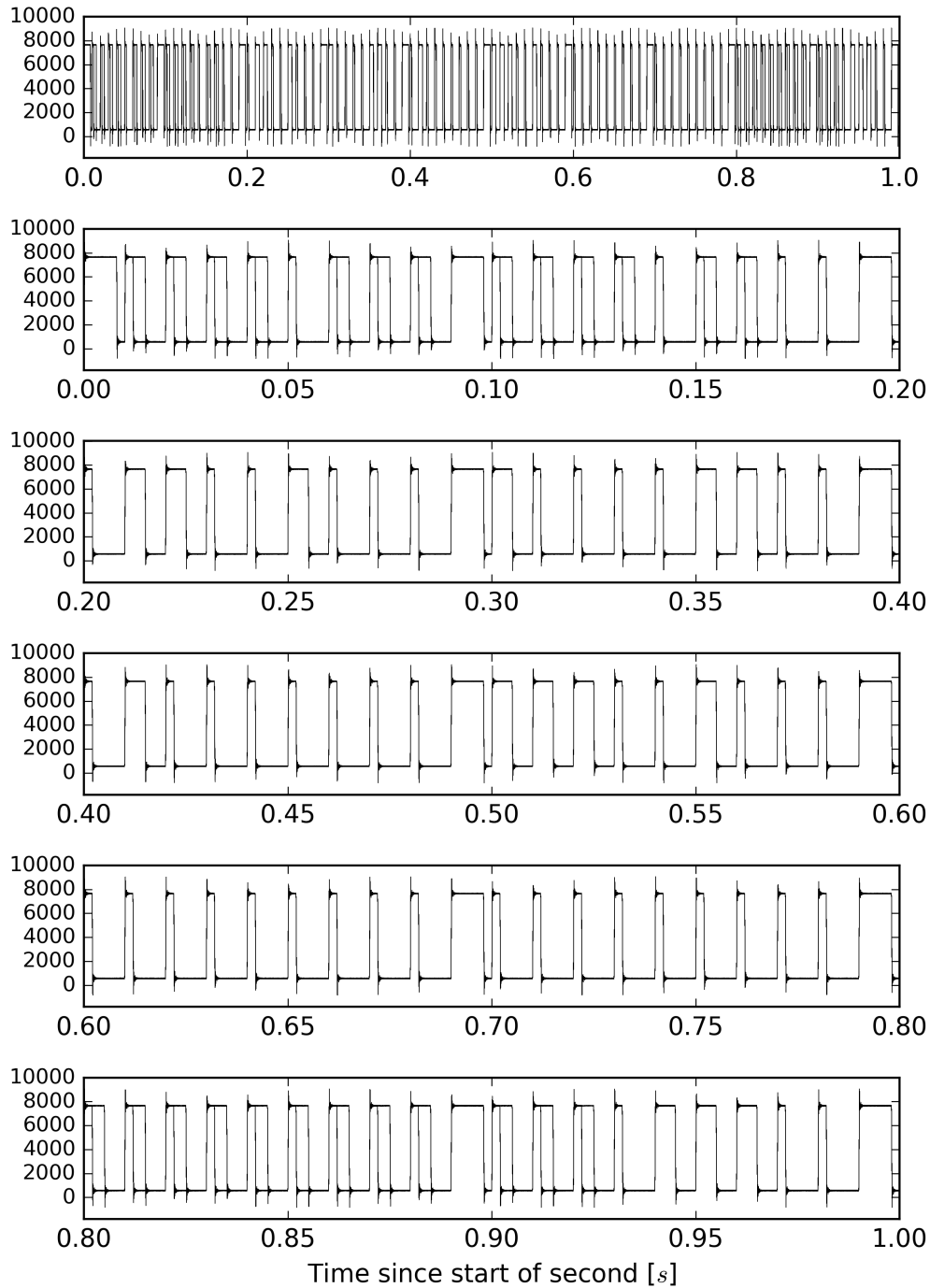
Overlay of H1:CAL-PCALX_IRIGB_OUT_DQ from 1187195763 to 1187195764
