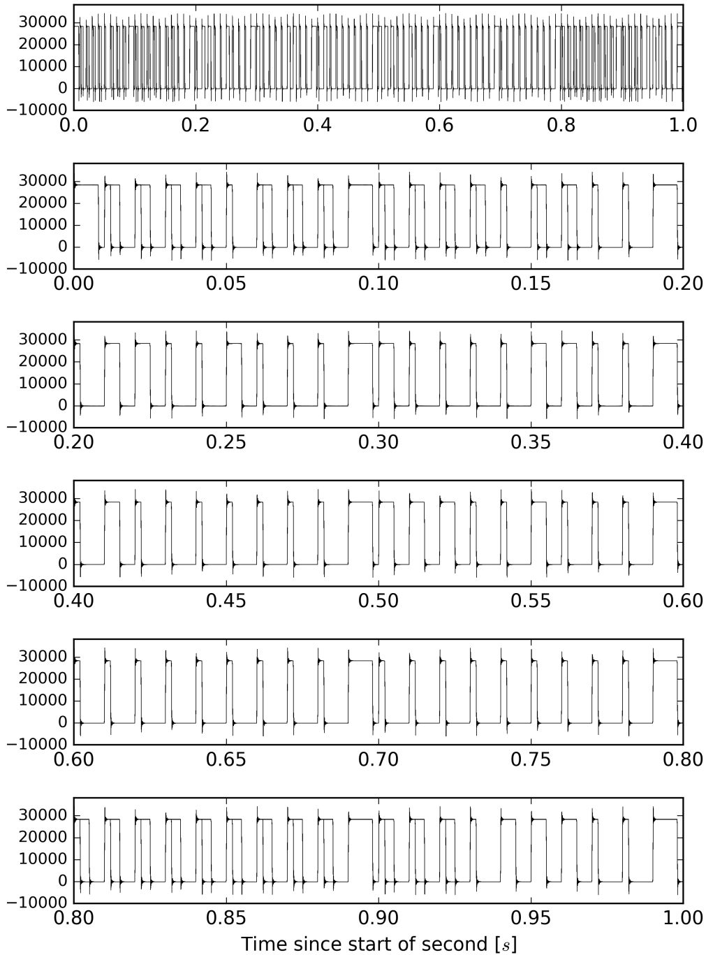
Overlay of L1:CAL-PCALY_IRIGB_OUT_DQ from 1187195763 to 1187195764
