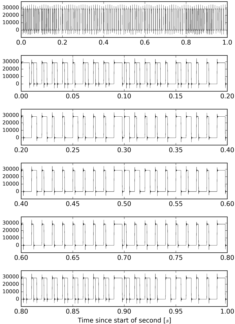
Overlay of L1:CAL-PCALX_IRIGB_OUT_DQ from 1187195763 to 1187195764
