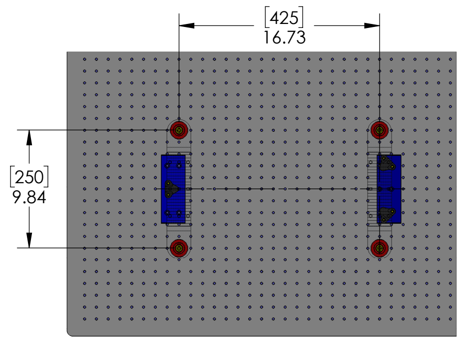
CROSS BAR LOCATIONS WRT KINEMATIC MT.
