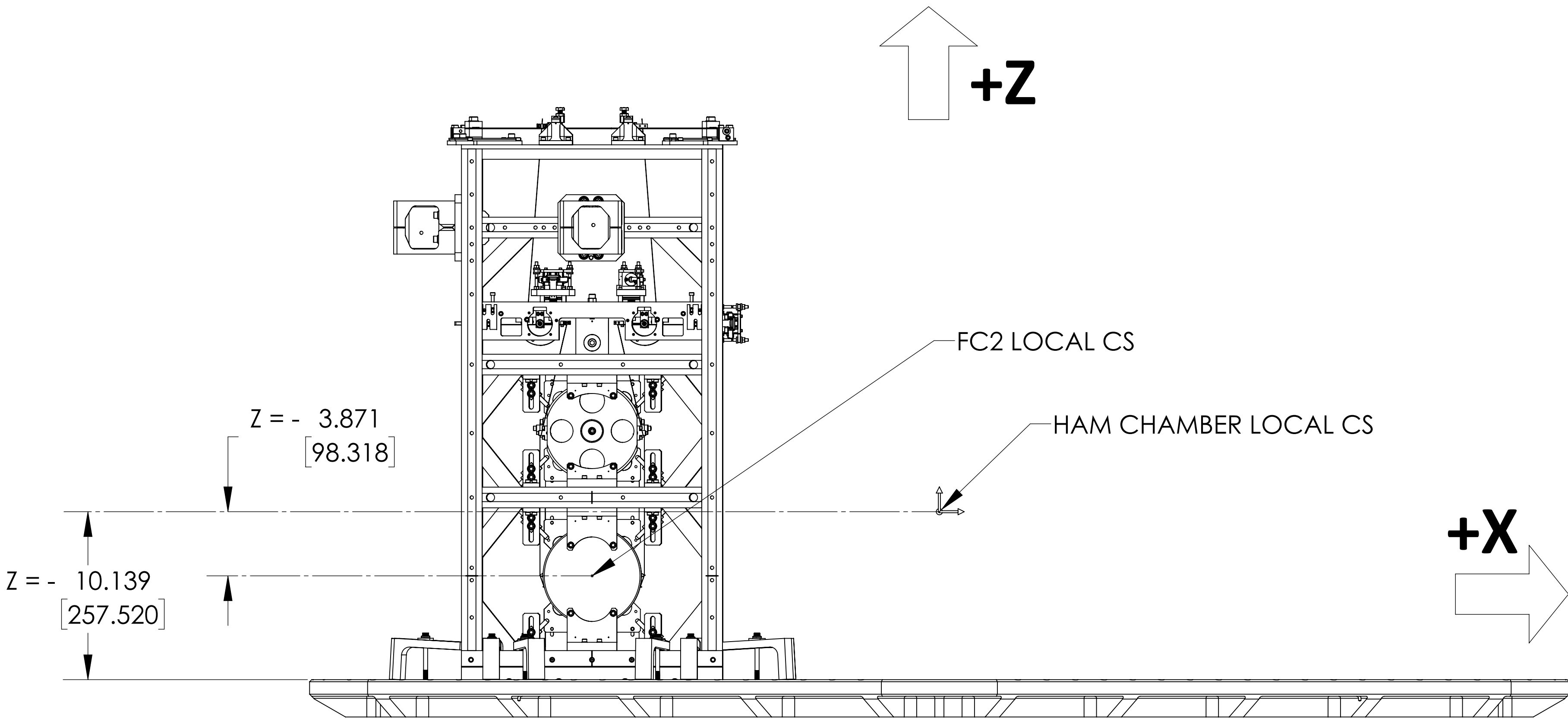
FRONT VIEW (BAFFLE AND CABLE ASSEMBLIES NOT SHOWN)
