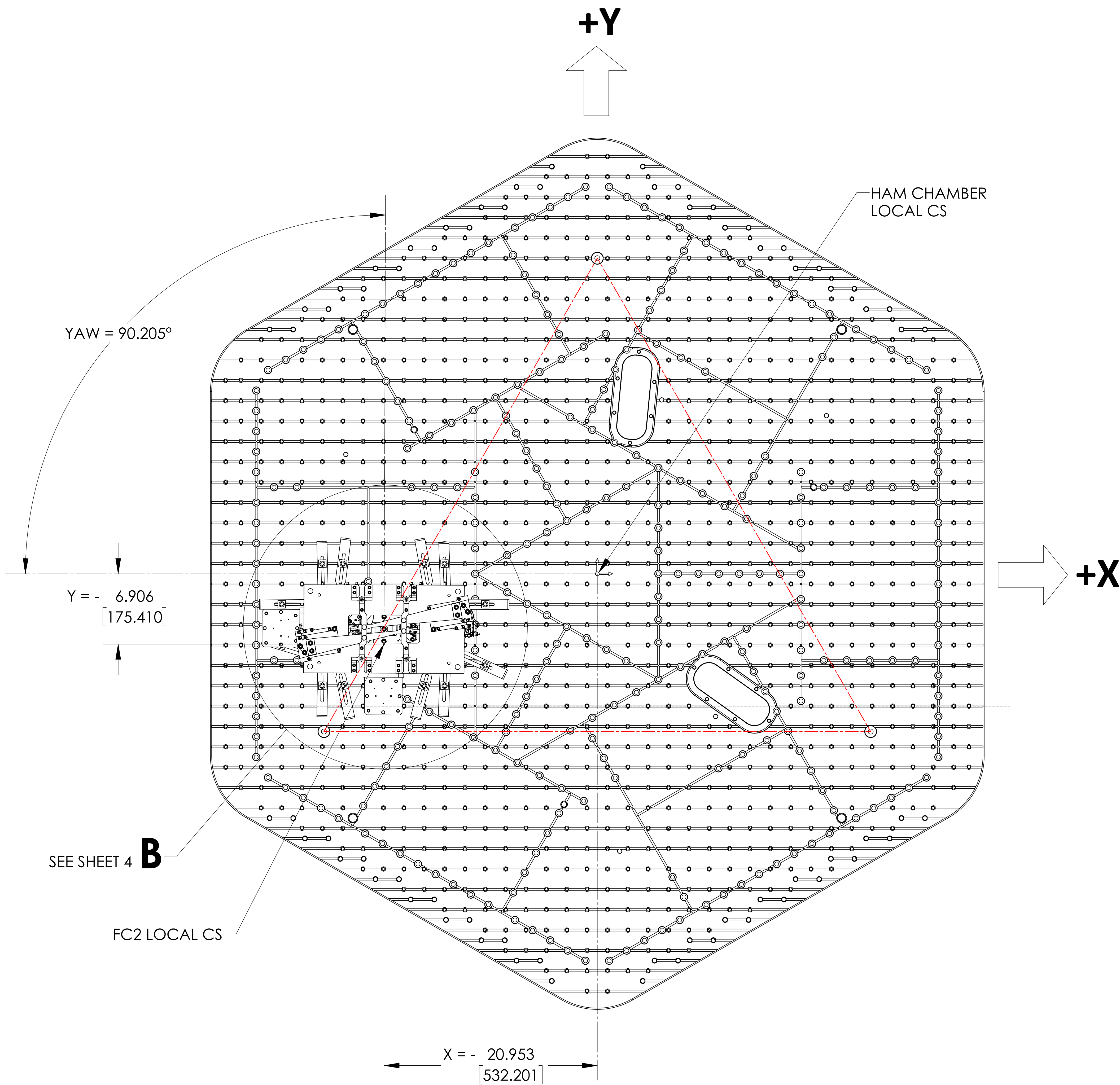
TOP VIEW (BAFFLE AND CABLE ASSEMBLIES NOT SHOWN)
