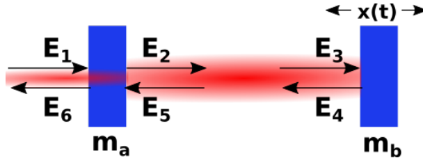
Figure 2.2. Simple cavity with labeled fields.
