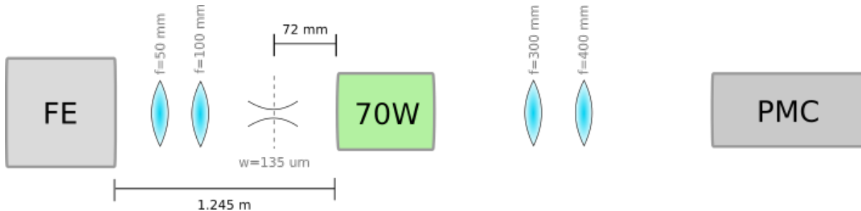
Figure 3.5. Diagram of the Front End to PMC modermatching layout.
