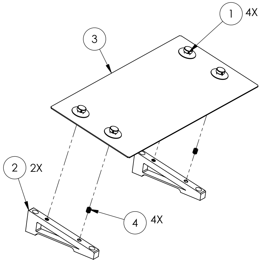
ISO VIEW (EXPLODED VIEW)
