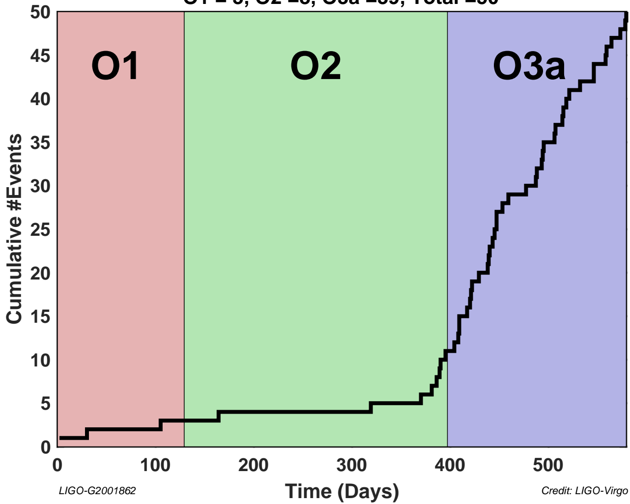
Cumulative Count of Events O1 = 3, O2 = 8, O3a = 39, Total = 50
