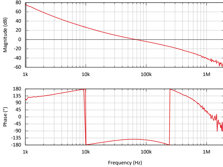
Fig. 13. The open loop transfer function of the power stabilization is designed to operate with a bandwidth of 70 kHz for best noise performance and high robustness.
