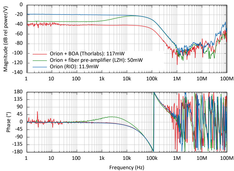
Fig. 8. The seed power is modulated to measure the transfer function to the output power of the pre-amplifiers. The seed power modulation (blue curve) is transferred to the output of the pre-amplifiers (green and red curves).
