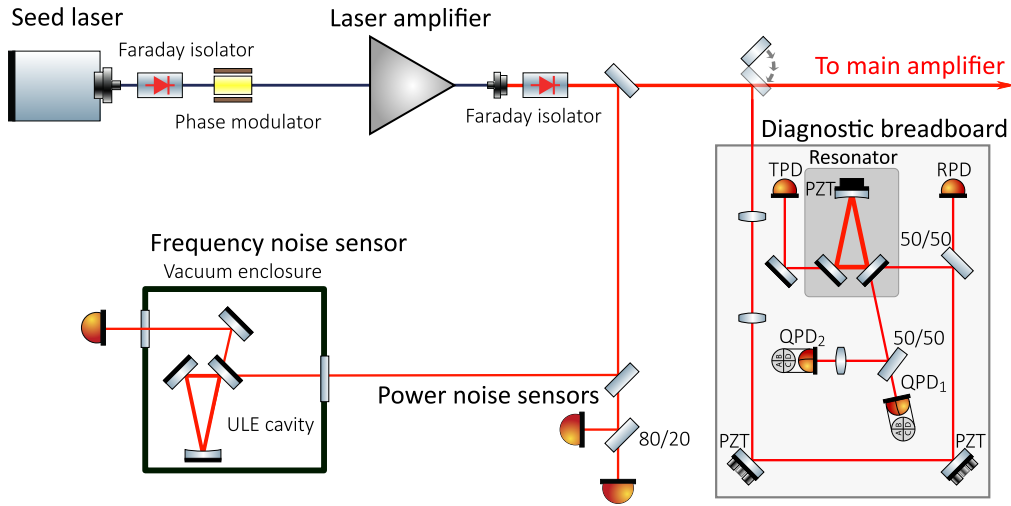
Fig. 1. The simplified stabilization setup shows the seed laser with 1550 nm wavelength, which was coupled via a fiber Faraday isolator to the fiber phase modulator and was amplified by the semiconductor booster amplifier. A Faraday isolator was placed in the 115 mW free space beam. This was to prevent reflections back to the amplifier. Parts of the beam were sent to power sensors and the frequency reference cavity. The main fraction of the beam was analysed with the diagnostic breadboard.
