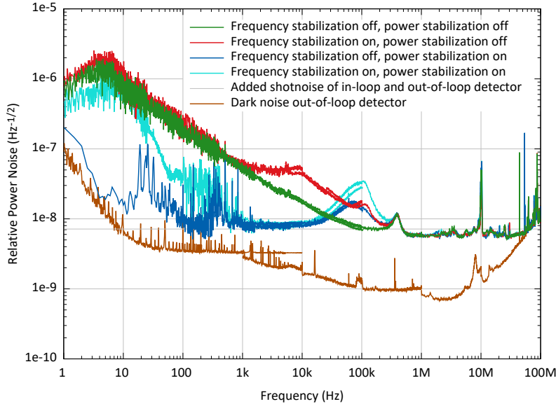
Fig. 14. The RPN as an amplitude spectral density was measured for several combinations of on/off states of the frequency and power stabilization control loops. A cross-coupling between frequency stabilization to power noise is visible.
