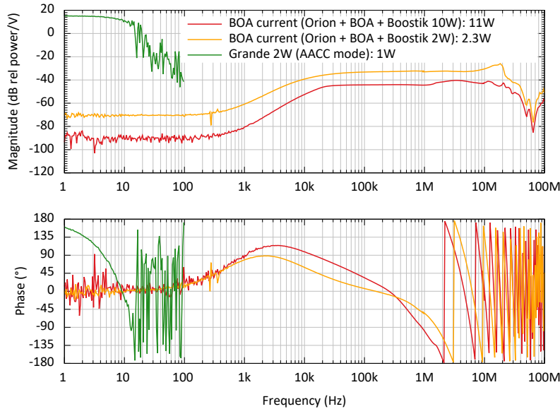
Fig. 10. The transfer functions from seed power modulations to power modulations of the power amplifier output power have the same shapes as the measurements with the fiber pre-amplifiers in Fig. 7.
