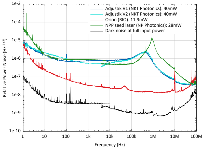
Fig. 3. The free-running RPN of the seed lasers, plotted as amplitude spectral density, follow two characteristic shapes. The Orion laser has a very low free-running noise, the fiber lasers have a higher noise floor and a characteristic relaxation oscillation peak.
