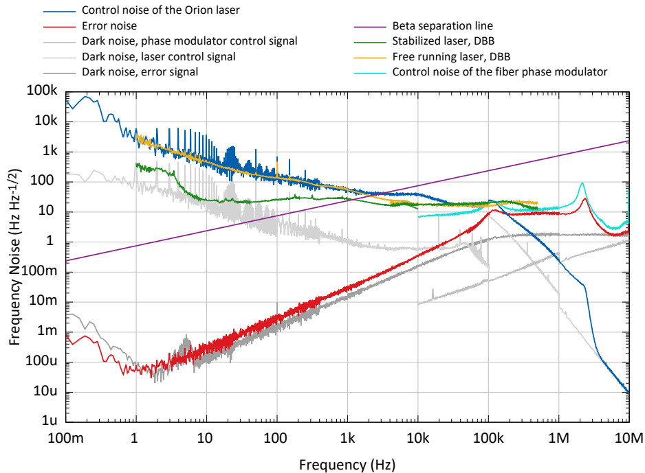
Fig. 12. The calibrated control signal noise (blue) and the calibrated error signal noise (red) are plotted for the frequency stabilization.
