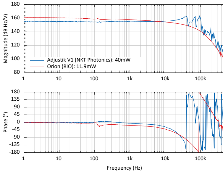
Fig. 4. The frequency actuation transfer functions of the fiber based and Orion laser show a similar magnitude at low frequencies. Resonances in the fiber laser's transfer function reduce the usable actuation bandwidth significantly compared to the Orion laser.
