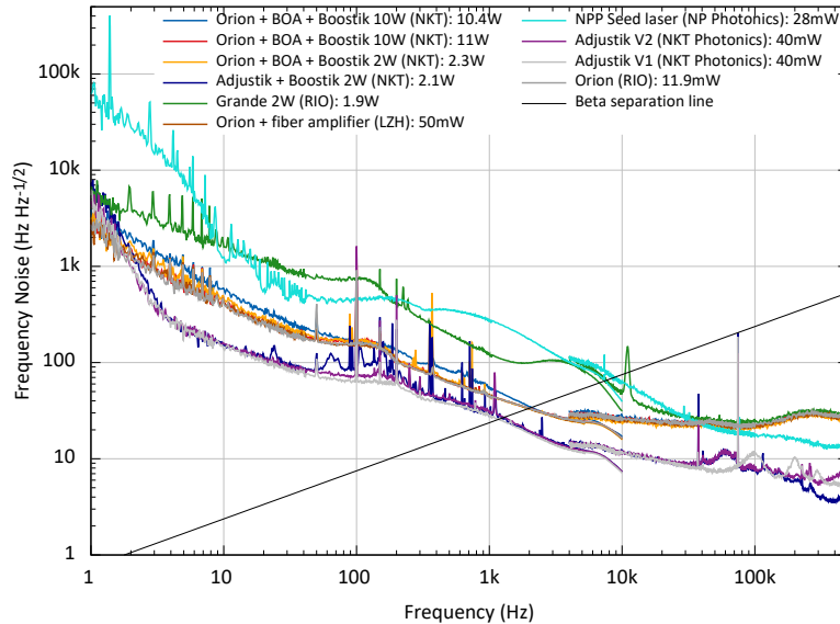
Fig. 2. The free-running frequency noise of the different seed lasers and MOPA combinations. The frequency noise of the MOPA systems is dominated by their seed laser noise.
