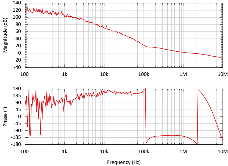
Fig. 11. The open loop transfer function of the frequency stabilization to the resonance frequency of the reference cavity is shown. A unity gain bandwidth of 1.3 MHz was achieved by utilizing a cross-over between seed laser and fiber phase modulator at 100 kHz.
