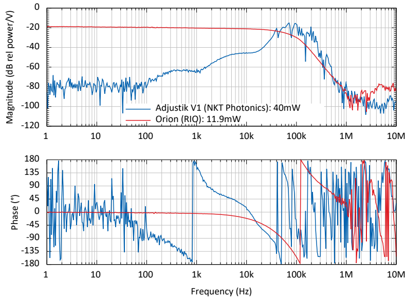
Fig. 5. The cross-couplings from frequency actuation to the output power of the Orion laser and fiber laser. As the pump current for the Orion laser also defines the output power, a direct coupling is observed. Meanwhile the output power of the fiber laser shows a strong coupling only around 70 kHz.
