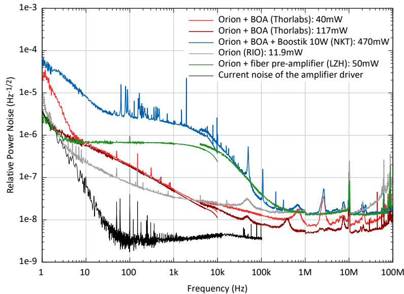
Fig. 6. The free-running RPN at the output of the pre-amplifiers is shown. For all measurements the Orion laser is used as the seed source (grey curve).
