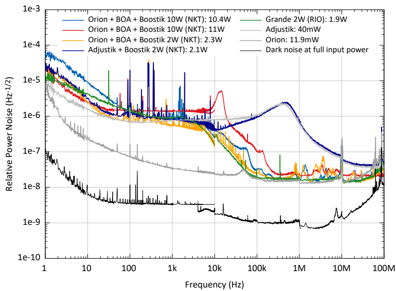
Fig. 9. The free-running RPN spectral densities at the output of the power amplifiers. At low frequencies the power noise of the amplifiers is dominated by their pump power noise.
