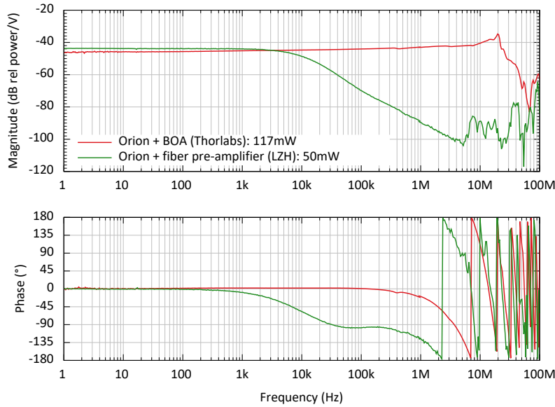
Fig. 7. The pump current of the BOA and fiber pre-amplifier's pump diodes is modulated to measure the transfer function to the pre-amplifier's output power.
