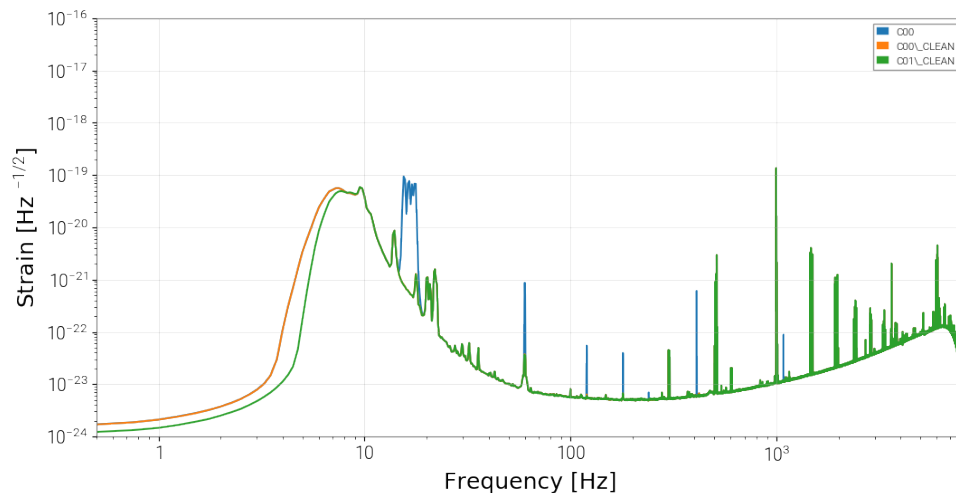
FIG. 5: Amplitude spectral density (ASD) comparison between the low-latency strain data with no cleaning applied (C00), the low-latency strain data with calibration lines and power mains lines removed (C00_CLEAN), and the high-latency strain data with calibration lines and power mains lines removed (C01_CLEAN).
