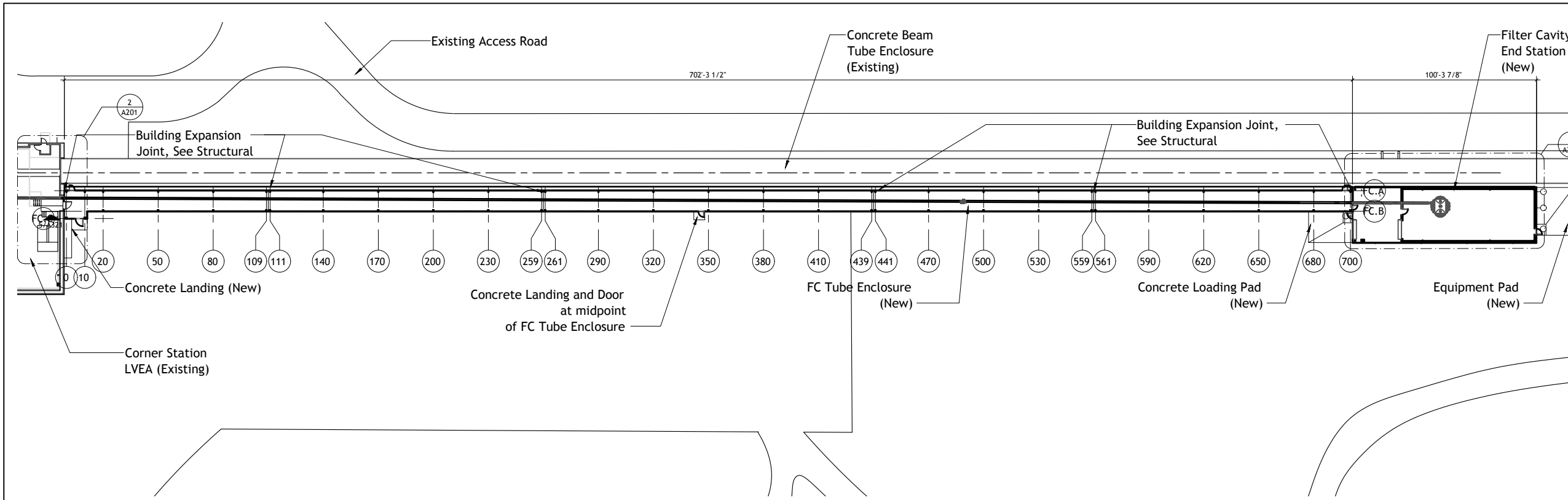
1 OVERALL PLAN A200 1/32" = 1'-0"
