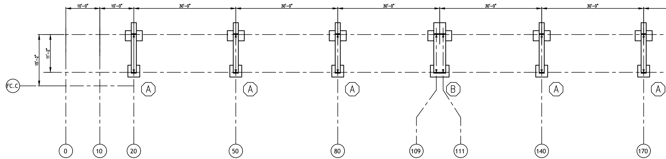
1 FC TUBE ENCLOSURE A - FOUNDATION PLAN S100 1/8" = 1'-0"
