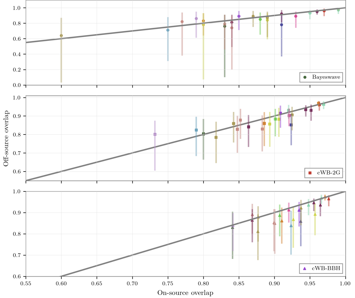
Figure 8. A comparison of the the overlap between the on-source and off-source (with 90% confidence intervals) reconstructions for three different minimally modeled pipelines, BAYESWAVE, CWB-2G, and CWB-BBH for candidates which had data from both interferometers and where the NRSUR7DQ4 waveform was used in parameter estimation, the network SNR was greater than 10, and the redshifted chirp mass (1+z)\mathcal{M} > 15M_{\odot} . The gray line denotes equal overlap between the on- and off-source reconstructions, indicating that there is no significant difference between the two.
