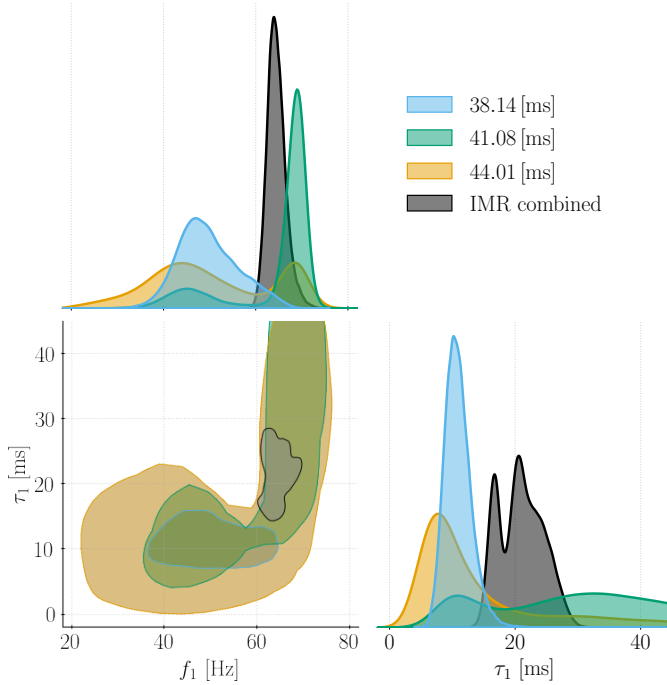
Figure 5. Two-dimensional frequency and damping time posterior distribution (90% credible levels), when starting the analysis at late times and assuming a single damped sinusoid with positive frequency; the combined IMR estimates for the longest-lived \ell mn = 220 QNM are shown for comparison. For visualisation purposes, we display up to \tau_1 = 45\text{ms} , while the posterior tail extends up to \tau_1 = 80\text{ms} .
