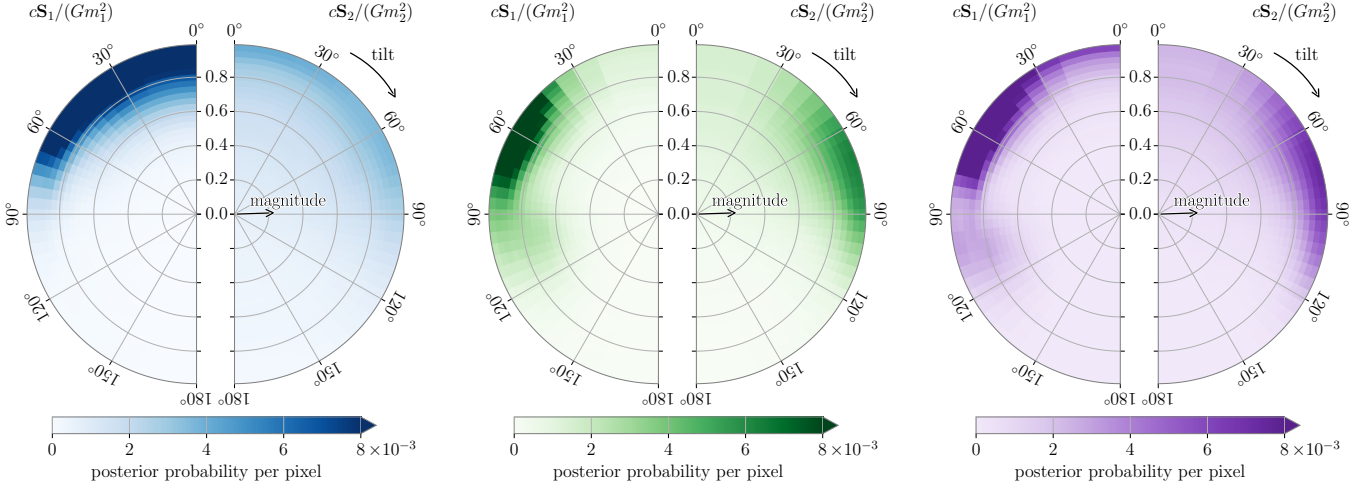
Figure 9. Posterior probabilities for the dimensionless component spins, cS_1/(Gm_1^2) and cS_2/(Gm_2^2) , relative to the orbital angular momentum axis \hat{L} . From left to right, we compare the posterior probabilities obtained when analysing LIGO Hanford data only (blue), LIGO Livingston data only (green), and a coherent analysis of LIGO Hanford and LIGO Livingston data (purple). In all cases, we show the posterior distribution resulting from equally combining samples from five waveform models. The tilt angles are 0^\circ for spins aligned with the orbital angular momentum and 180^\circ for spins anti-aligned. Probabilities are marginalized over the azimuthal angles. The pixels have equal prior probability, being equally spaced in the spin magnitudes and the cosines of tilt angles. The spin orientations are defined at a fiducial GW frequency of 10 Hz.
