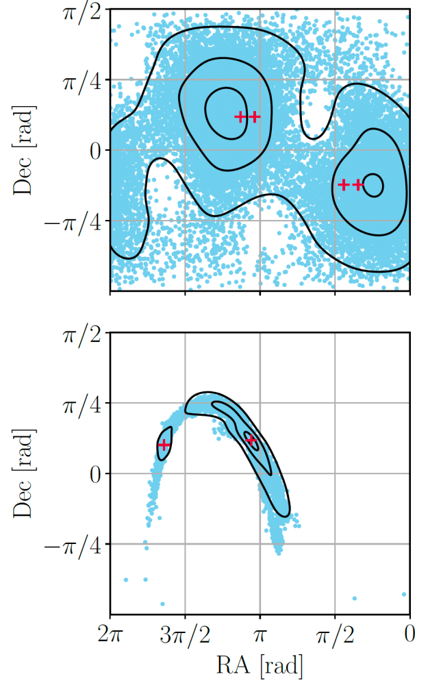
Figure 1. Joint RA and Dec posterior distribution for the merger remnants from GW230814 (top) and GW231123 (bottom). The black contours show the 90%, 50%, and 10% confidence intervals. The red crosses indicate the sky positions targeted in the search for each remnant.
